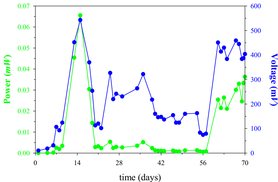
Fig. 2 Power and voltage of the double chamber MFC. Catholyte concentration was increased on day 15 and changed every 7 days, and polarisation was carried out on day 22
