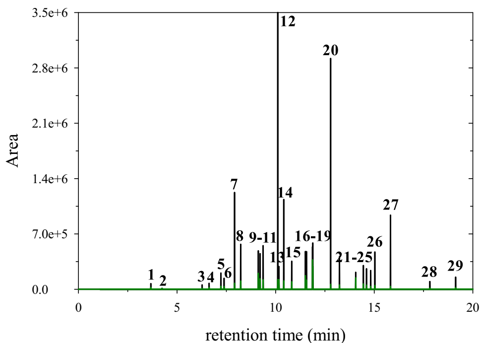
Fig. 5 Total Petroleum Hydrocarbons (TPHs) total ion chromatogram where 29 TPHs were detected in OW ( black ) and MFC anolyte before the feed replacement with OW ( green ). Peaks 1–29 correspond to TPHs listed in Table 1
