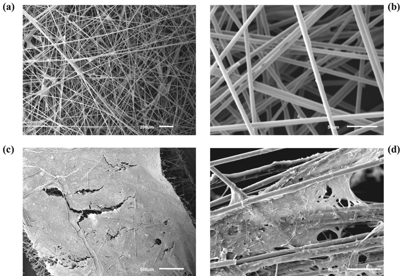
Fig. 4 SEM images a 200 \mu\text{m} and b 50 \mu\text{m} of a blank electrode, c 500 \mu\text{m} and d 50 \mu\text{m} of the anode electrode surface after 70 days of MFC operation with OW
