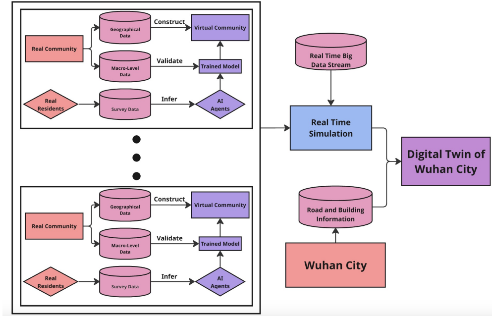
Figure 5: Framework of Real-Time Urban Digital Twin Construction Based on Multi-Source Data: The Case of Wuhan Large-Scale Social Simulator
