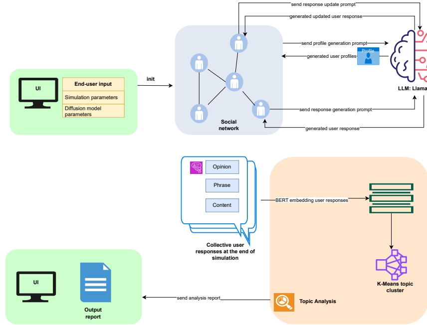
Figure 3: LLM-AIDSim Framework (Zhang et al. 2025)
