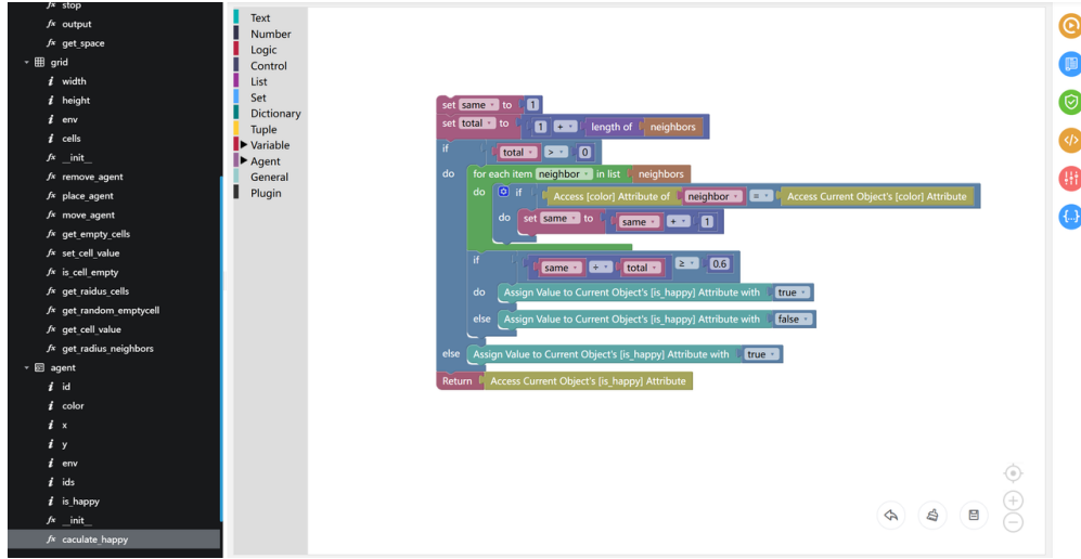
Figure 2: The Blocks of the Schelling Model at AgentBlock.net available from this link .
