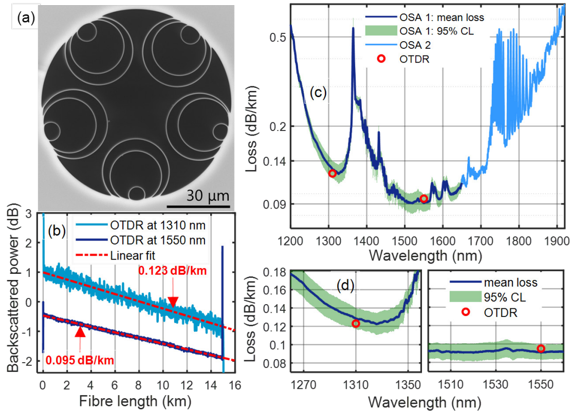
Fig.2: Characterisation of the fabricated fibre. (a) SEM of the fabricated HCF2; (b) bi-directional OTDR traces at 1310 and 1550 nm; (c) mean loss and 95% confidence level of four separate cutbacks (1200-1650 nm) compared to OTDR results and a fifth cutback to show the spectral loss in the 1650-1950 nm range; (d) cutback loss details in the 1270-1350 nm and 1500-1560 nm bands.
