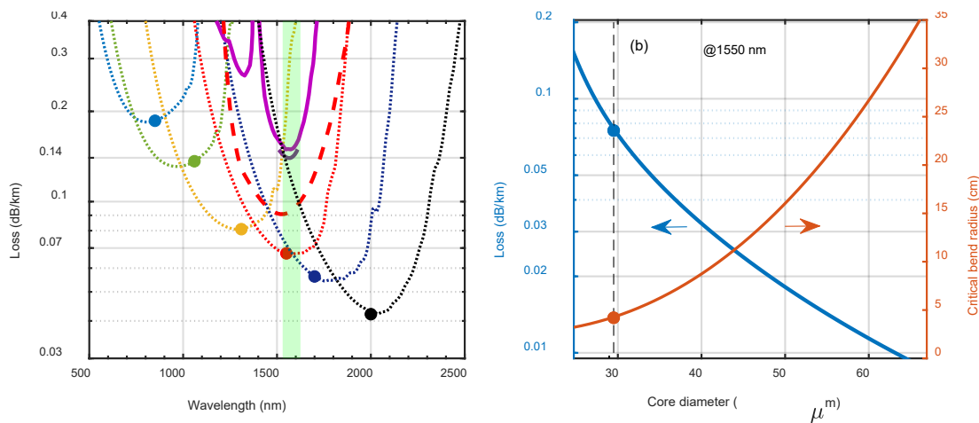
Fig.4: Simulated potential performance of further optimised fibres. (a) Loss of state-of-the-art PSCFs (pink and purple, see Fig.2), compared to loss of HCF2 (red dashed, gas absorptions omitted) and ideal DNANF with perfect structure (red dotted). The other dotted curves are modelled losses (sum of leakage, surface scattering and microbend loss contributions) of DNANFs with core and tube thicknesses optimised for guidance at 850, 1060, 1310, 1700, and 2000 nm; (b) total simulated loss and critical bend radius as a function of core diameter for a 1550 nm fibre similar to HCF2 with suitably larger core diameter and thicker coating.
