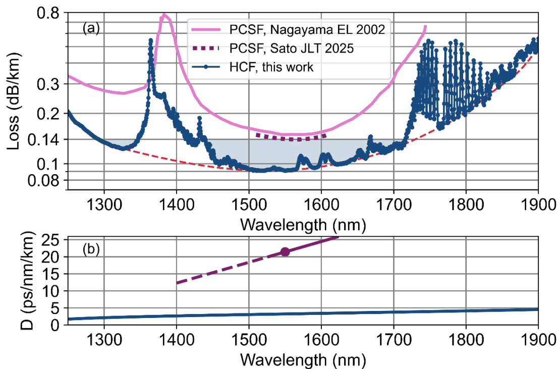
Fig.3: Loss and chromatic dispersion comparison with state-of-the-art telecoms fibres. (a) Loss of the DNANF in this work, compared with that of the record-low loss pure silica core fibres (PSCFs) from 2002 (Nagayama et al. 34 ) and 2025 (Sato et al. 10 ); (b) simulated dispersion of the DNANF and measured dispersion of the PSCF from Sato et al.
