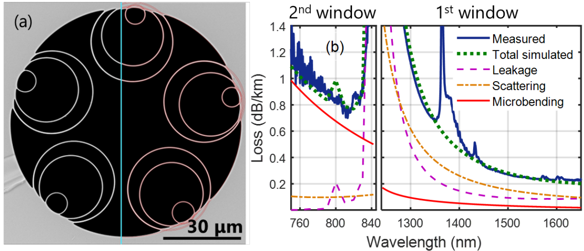
Fig. 1: Modelling validation. (a) Scanning Electron Microscope (SEM) image of the cross-section of one of the DNANFs used to calibrate our loss model. In red the automatic edge extraction of the tubular resonators used to inform simulations; (b) measured loss of the same fibre and simulation of its leakage loss (LL), surface scattering loss (SSL) and microbend loss ( \mu BL). The total simulated loss shows good agreement with the measurement in both the first (left) and second (right) antiresonant windows, despite being dominated by different mechanisms.
