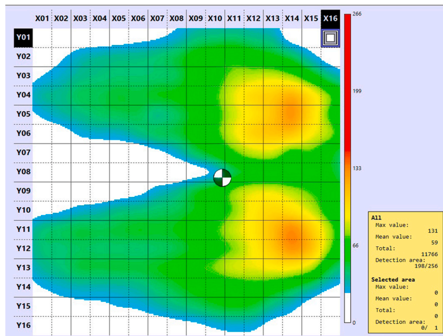
Fig. 17. Pressure mapping.
