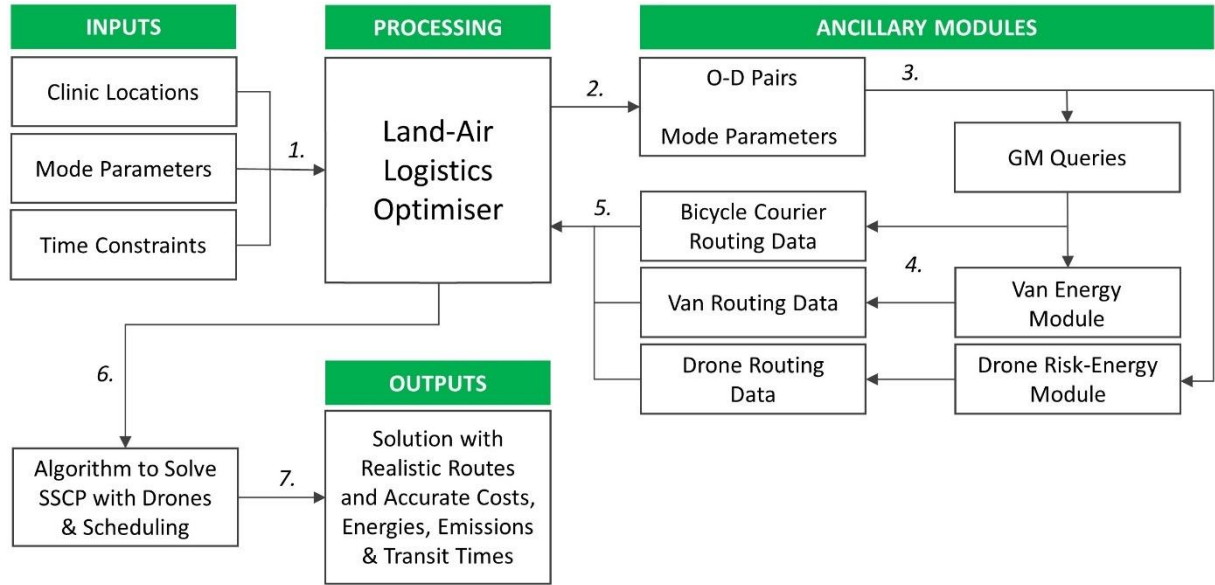
Figure 1. Diagram of the FORSETI logistics planning tool. Numbers indicate step sequence. O-D is origin-destination. GM is Google Maps. SSCP is Sustainable Specimen Collection Problem.
