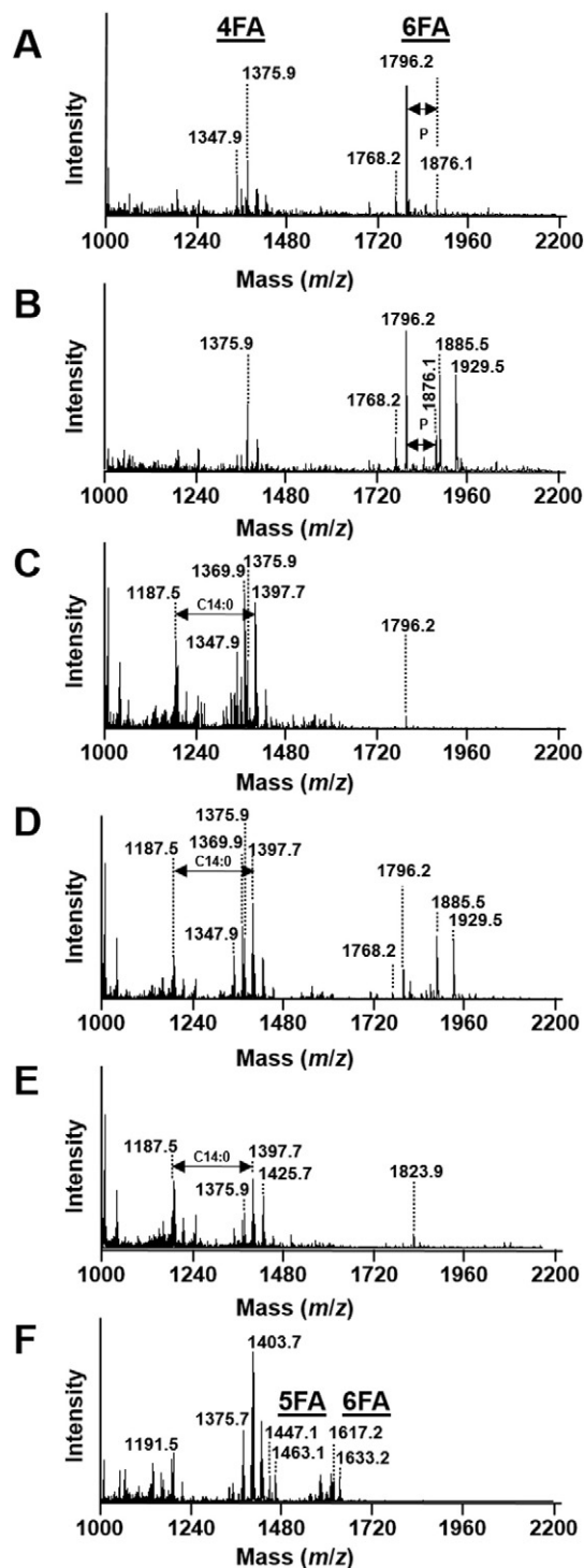
Fig. 1. Negative ion mode MALDI-TOF MS spectra of intact heat-inactivated S. sonnei (A), S. flexneri (B), enterohemorrhagic E. coli (C), enteroinvasive E. coli (D), K. pneumonia (E), P. aeruginosa (F). (FA: fatty acid).
