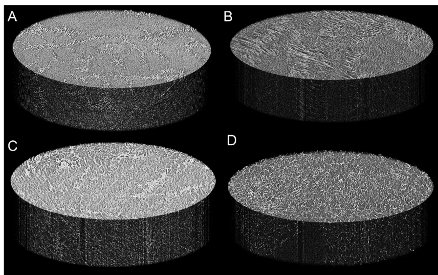
Fig. 2. Representative, three-dimensional, reconstructions of micro-CT images of the developed aerogels. Light coloured portions of the material indicate a higher density. Aerogels prepared with 10% PVA solution (A) show areas of more tightly packed fibres and large areas of more even density suggesting a high a degree of structural heterogeneity within the gel. Aerogels made with 7.5% PVA (B) exhibited similar structure to 10% aerogels. Areas of varying material density were seen in 5% aerogels (C) and 1% aerogels (D) though a greater overall level of homogeneity was apparent in these. Images are representative of 3 independent replicates.
