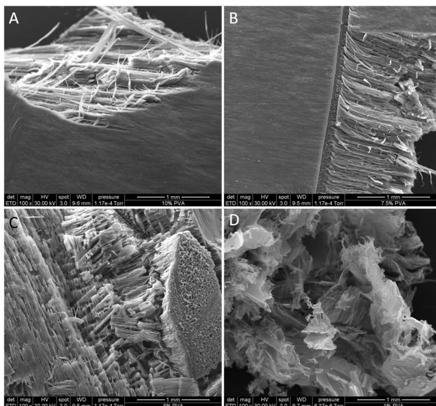
Fig. 1. Scanning electron micrographs of aerogels with varying PVA concentration. (a) 10% PVA aerogel (b) 7.5% PVA aerogel (c) 5% PVA aerogel (d) 1% PVA. High levels of fibre organisation are seen in the higher concentration PVA gels with lower fibre organisation in the lower concentration PVA gels.
