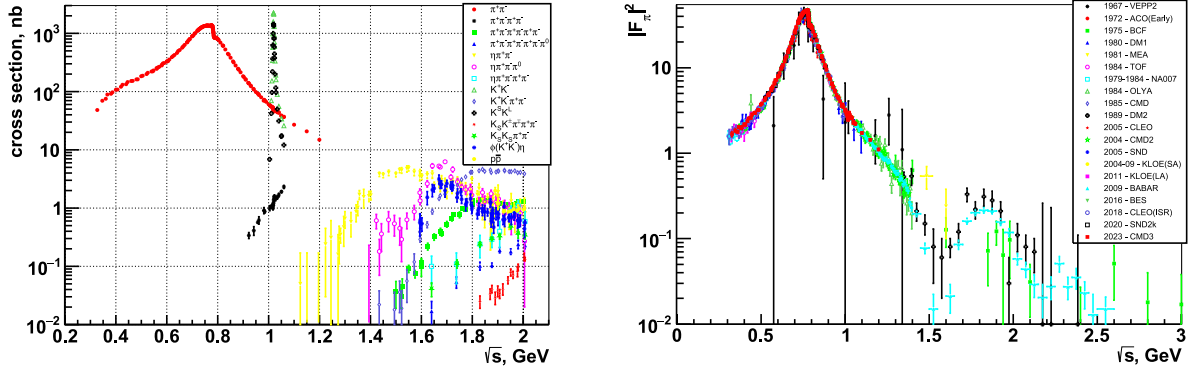
Fig. 1. Left: Published measurements of e^+e^- \rightarrow \text{hadrons} cross sections by the CMD-3 experiment [95–108]. Right: Status of the e^+e^- \rightarrow \pi^+\pi^- cross-section measurement with different experiments contributing over the years [95,96,109–140].
