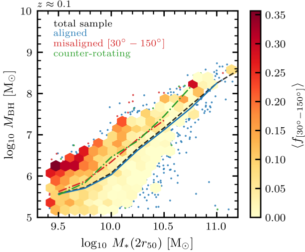
Figure 6. M_* – M_{\text{BH}} relation at z \approx 0.1 for a representative sample of galaxies with reliable kinematic measurements over 0.10 \lesssim z \lesssim 0.28 . Bins coloured according to the fractional time a galaxy spends in the unstable misaligned regime ( \langle f_{[30^\circ-150^\circ]} \rangle ) within this redshift range, averaged for all galaxies within a given bin (minimum count of 5). Medians are shown for the total sample (black dashed) and sub-samples of aligned (blue solid), unstable misaligned (red dash-dotted), and counter-rotating (green dash-dotted) galaxies for bins with a minimum bin count of 10. We find a strong correlation between galaxies hosting overmassive BHs and galaxies with a history of spending more time in the unstable misaligned regime.
