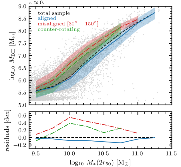
Figure 5. M_* - M_{\text{BH}} relation at z \approx 0.1 for galaxies in various stellar-gas kinematic states. Top: median lines for the total sample (black dashed) and sub-samples of aligned (blue solid), unstable misaligned (red dash-dotted), and counter-rotating (green dash-dotted) galaxies for bins with a minimum bin count of 10. Shaded regions show the 25 and 75 percentiles for aligned, unstable misaligned, and counter-rotating galaxies. Grey scatter points show the total sample. Bottom: residuals of aligned, unstable misaligned, and counter-rotating medians, with respect to the total sample. We find overmassive BHs preferentially reside in galaxies that are currently in the unstable misaligned or counter-rotating regime, with a maximum BH mass difference of \sim 0.6 dex at a turnover mass of \sim 10^{10} M_\odot .
