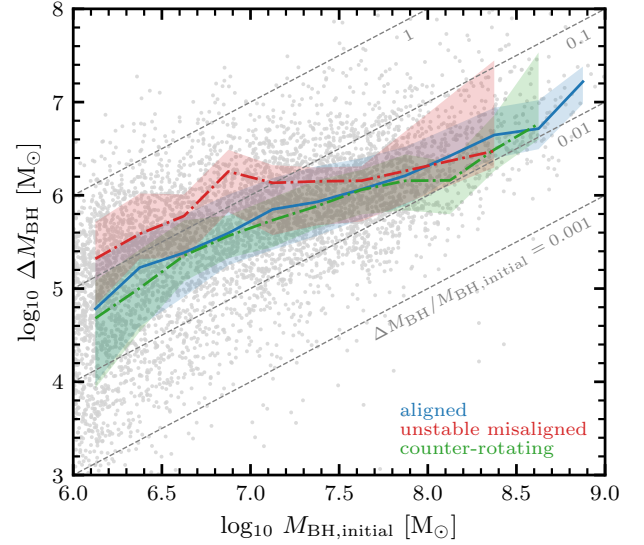
Figure 1. Median change in BH mass traced over a 0.50 \pm 0.05 Gyr window as a function of the initial BH mass for samples of galaxies which are aligned (blue solid), counter-rotating (green dash-dotted), and galaxies experiencing an unstable misalignment (red dash-dotted). Shaded regions show the 25 and 75 percentiles. Grey scatter points show the total sample. Diagonal lines (dashed grey) show the relative increase in BH mass, with \Delta M_{\text{BH}}/M_{\text{BH,initial}} = 1 indicating a doubling of BH mass over this window. We find that counter-rotating galaxies exhibit similar BH growth to aligned galaxies, while galaxies experiencing an unstable misalignment show significantly higher ( \sim 0.6 dex) BH growth up to BH masses of M_{\text{BH,initial}} \gtrsim 10^{7.5} M_{\odot} .
