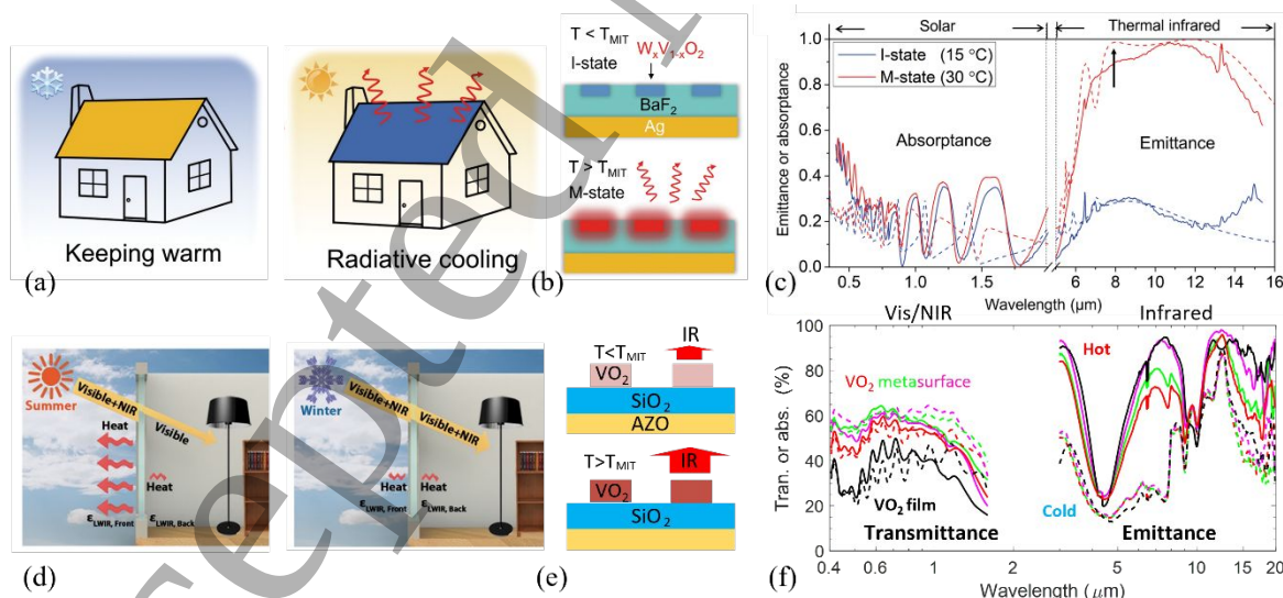
Figure 1. (a)–(c) Smart house roof with tunable radiative cooling: (a) schematic illustration; (b) \text{W:VO}_2 metamaterial reflector enabling tunable radiative cooling in insulating (I) and metallic states (M); (c) absorption spectra in the insulating and metallic states. (d)–(f) Smart windows with a tunable radiative cooling: (d) schematic illustration; (e) visible-transparent \text{VO}_2 metasurface integrated with an Al-doped zinc oxide (AZO); (f) transmission and absorption spectra in insulating and metallic states. Reproduced with permission from [5–7].
