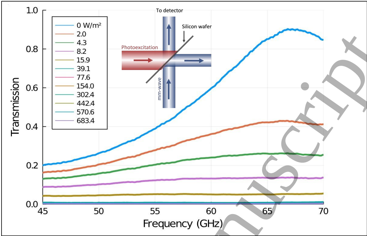
Figure 1. The transmission as a function of frequency through a 1 k \Omega .cm, 675 \mu m thick, silicon wafer that has had its surfaces passivated with Al_2O_3 to increase the charge carrier lifetime. The transmission through the wafer on Fabry P  rot resonance is reduced by >90% when the Si is photoexcited with approximately 10 W/m^2 of optical light - just 1/100th of strong daylight [5].
