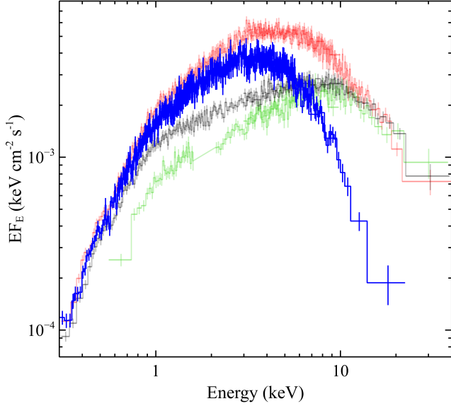
Figure 2. The broadband spectrum of one of the new soft state observations of Holmberg IX X-1 (epoch 7; solid blue), compared to the three broadband spectra highlighted by Walton et al. (2017a) that are representative of the archival observations (epochs 1, 2 and 4; faded black, red and green, respectively). For clarity, we only show the NuSTAR data from FPMA along with one of the accompanying soft X-ray detectors (either the EPIC-pn data for XMM-Newton or the FI XIS data for Suzaku ). Of the four other new broadband epochs presented in this work, epochs 8 and 9 are similar to epoch 7 (blue), epoch 10 is similar to epoch 2 (red), and epoch 11 is similar to epoch 1 (black). All the data have been unfolded through the same model, which is simply constant with energy, and the data have been further rebinned for visual purposes.
