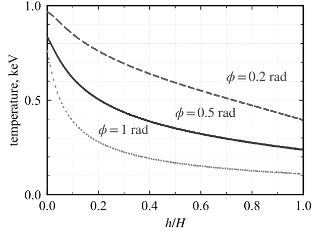
Figure 5. Temperature profiles over the cavity walls for different opening angles (see Section 3.3). The temperature distribution over the walls of the accretion cavity. Different curves are shown for different opening angles of the cavity: \phi = 0.2 rad, 0.5 rad, and 1 rad (from top to bottom). The temperature of the walls tends to increase towards the accretion disc plane. The smaller the opening angle, the higher the temperature of the walls. Parameters: L = 5 \times 10^{39} erg s ^{-1} , R_m = 5 \times 10^7 cm, H/R_m = 10 .
