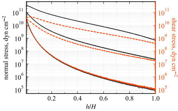
Figure 3. Radiation-induced stress on the cavity walls (see Section 3.2). The normal (black solid lines) and shear (red dotted lines) stress at the walls of the accretion cavity. Different curves are given for different opening angles of the cavity (from bottom to top): \phi = 1 rad, 0.5 rad, 0.2 rad. The smaller the opening angle, the larger the stress at the walls. Parameters: L = 5 \times 10^{39} erg s ^{-1} , R_m = 5 \times 10^7 cm, H/R_m = 10 .
