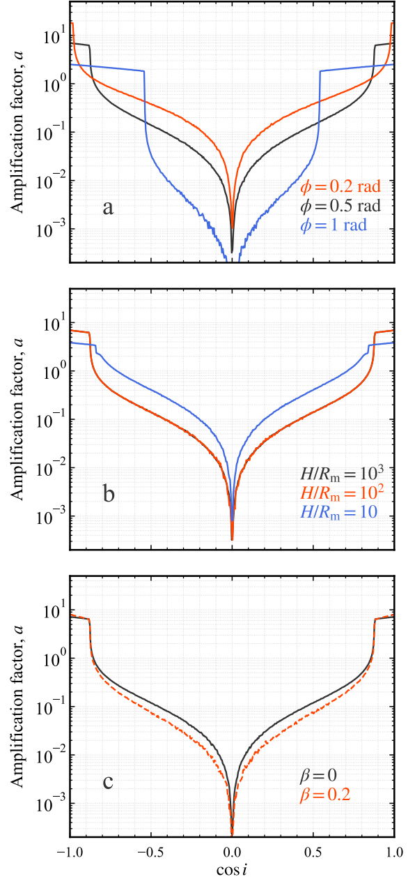
Figure 2. Angle-dependent geometrical beaming of the emission (see Section 3.1). The amplification factor as a function of observer inclination i with respect to the accretion cavity. (a) The accretion cavity relative height and wall velocity are fixed at H/R_m = 10^3 and \beta = 0 . Different curves correspond to various opening angles of the cavity: 1 rad (blue line), 0.5 rad (black line), 0.2 rad (red line). (b) The opening angle and wall velocity are fixed at \phi = 0.5 \text{ rad} and \beta = 0 . Different curves correspond to varying relative heights of the accretion cavity: H/R_m = 10^3 (black line), H/R_m = 10^2 (red line), H/R_m = 10 (blue line). (c) The relative height and opening angle are fixed at H/R_m = 10^3 and \phi = 0.5 \text{ rad} . Different curves correspond to different velocities of the accretion cavity walls: \beta = 0 (black solid line), \beta = 0.2 (red dashed line).
