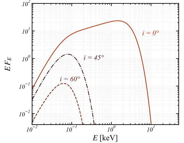
Figure 7. Angle dependence of the reprocessed spectrum from the accretion cavity. Model parameters: L = 5 \times 10^{39} \text{ erg s}^{-1} , R_m = 10^8 \text{ cm} , H/R_m = 10^3 , \phi = 0.5 \text{ rad} , and \beta = 0 . Curves show observer inclinations i = 0^\circ (solid), 45^\circ (dash-dot), and 60^\circ (dashed), i.e. a “low vs. high inclination” view. The high-energy part hardens strongly toward lower i (greater visibility of hotter wall regions near the disc plane), while the soft flux varies comparatively little with inclination. Only the reprocessed component is shown; direct pulsar emission is not included.
