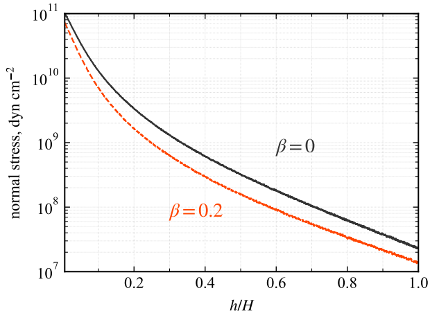
Figure 4. Effect of wall motion on the normal stress (cf. Fig. 3). Normal stress at the walls of the accretion cavity calculated for different wall velocity: \beta = 0 (black solid line) and \beta = 0.2 (red dashed line). One can see that including effects of special relativity reduces the stress by a factor \sim 2 for the case of \beta = 0.2 . Parameters: L = 5 \times 10^{39} erg s ^{-1} , R_m = 5 \times 10^7 cm, H/R_m = 10 , \phi = 0.5 rad.
