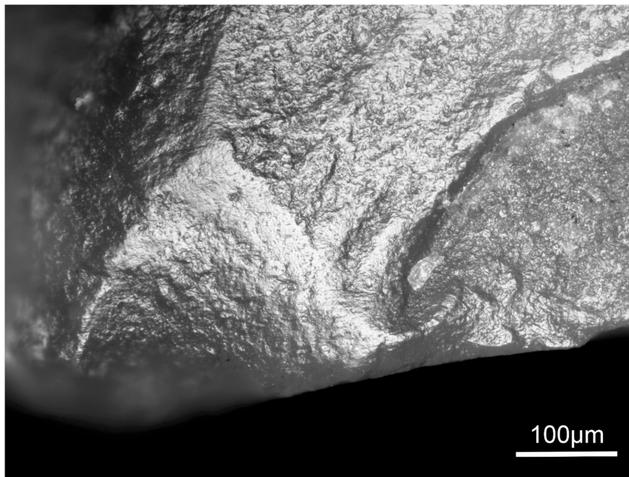
Fig. 9. Longitudinal polish on the edge of Object 14 at 200x magnification (scale bar is 100 µm).
