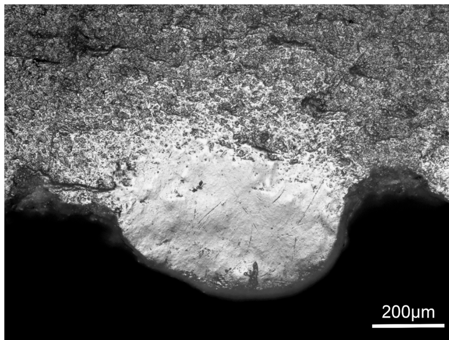
Fig. 7. The distribution of B-side polish on the teeth of Object 17 at 100x magnification (scale bar is 200 \mu\text{m} ).
