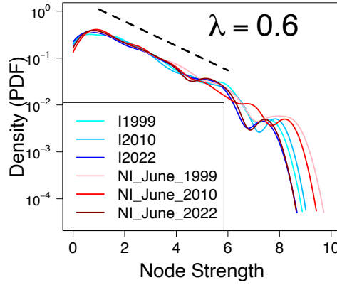
Fig. 4 Node strength distribution of the I and NI networks. An exponential distribution with decay rate \lambda = 0.6 with node strength s \in [1, 6] is plotted as the dotted line against the distributions.
