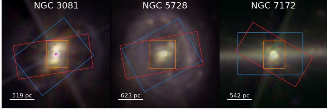
Figure 1. False colour JWST MIRI PSF-subtracted images of the three shared targets, NGC 3081, NGC 5728, and NGC 7172, covering a 15'' \times 15'' FoV around the nuclear point source. In these RGB images, the blue, green and red channels have been assigned to the JWST MIRI F1000W, F1500W and F1800W filters respectively. Overlaid on the images are the fields of view covered by SINFONI (orange, 3.3'' \times 3.8'' ), JWST/MRS (blue, 7.3'' \times 9.0'' ), and Spitzer/IRS (red, 11.3'' \times 4.7'' ).
