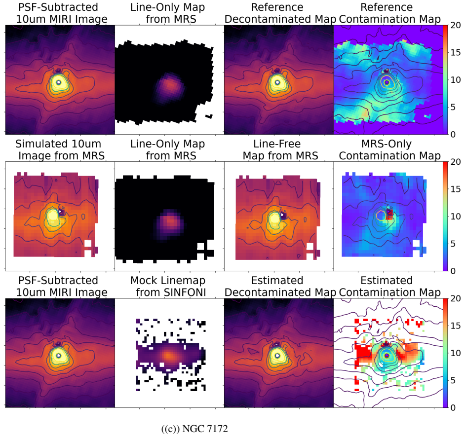
Figure 4. A summary of all three methods used on the three shared objects in F1000W – NGC 3081, NGC 5728, NGC 7172. The top row shows the reference method: the PSF-subtracted MIRI image is combined with the line-only MRS map, subtracting this gives the decontaminated map, and the contamination percentage map is the amount of flux from line emission compared with that in the PSF-subtracted image. The middle row shows the MRS-only method: the full image is synthesised from the MRS data, and can be decomposed into line-only emission and line-free emission. In this case, the synthetic line-free map is effectively the decontaminated image. The contamination map is the percentage of flux in the line-free map compared with the synthetic image. The bottom row shows the estimation method: The PSF-subtracted MIRI image is combined with a mock linemap generated from SINFONI data, subtracting this linemap from the image gives the estimated decontaminated map, and the contamination map is created through the ratio of the linemap flux to the image flux. The contours in these images, in all cases, represent the flux. The contours in the first column shows the flux in the image. The contours in the third column are that of the flux in the decontaminated map. The contours in the fourth column are those of the flux in the initial image.
