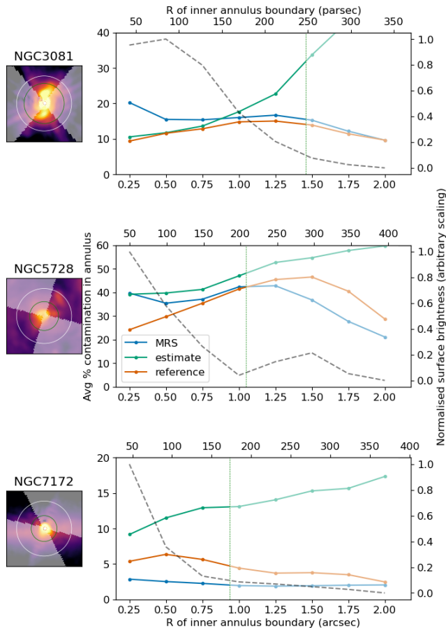
Figure 7. Radial average contamination percentage measured within sector covered by ionisation cone. On the left, we show thumbnails of the MIRI 10 \mu m images, with the regions outside the ionisation cone masked. The white circle indicates the 2 arcsec radius covered by the radial plot, and the green circle shows the radius at which the average flux reaches 10% of the peak
