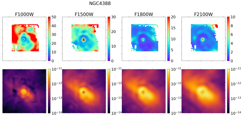
Figure C6. Contamination maps (top row) and line-free synthetic images (bottom row) shown across the 4 filters for NGC 4388. These were generated using the imaging-only estimation method described in Section 3.4, with the tracers used for the relevant lines in other bands described in Section C2.
