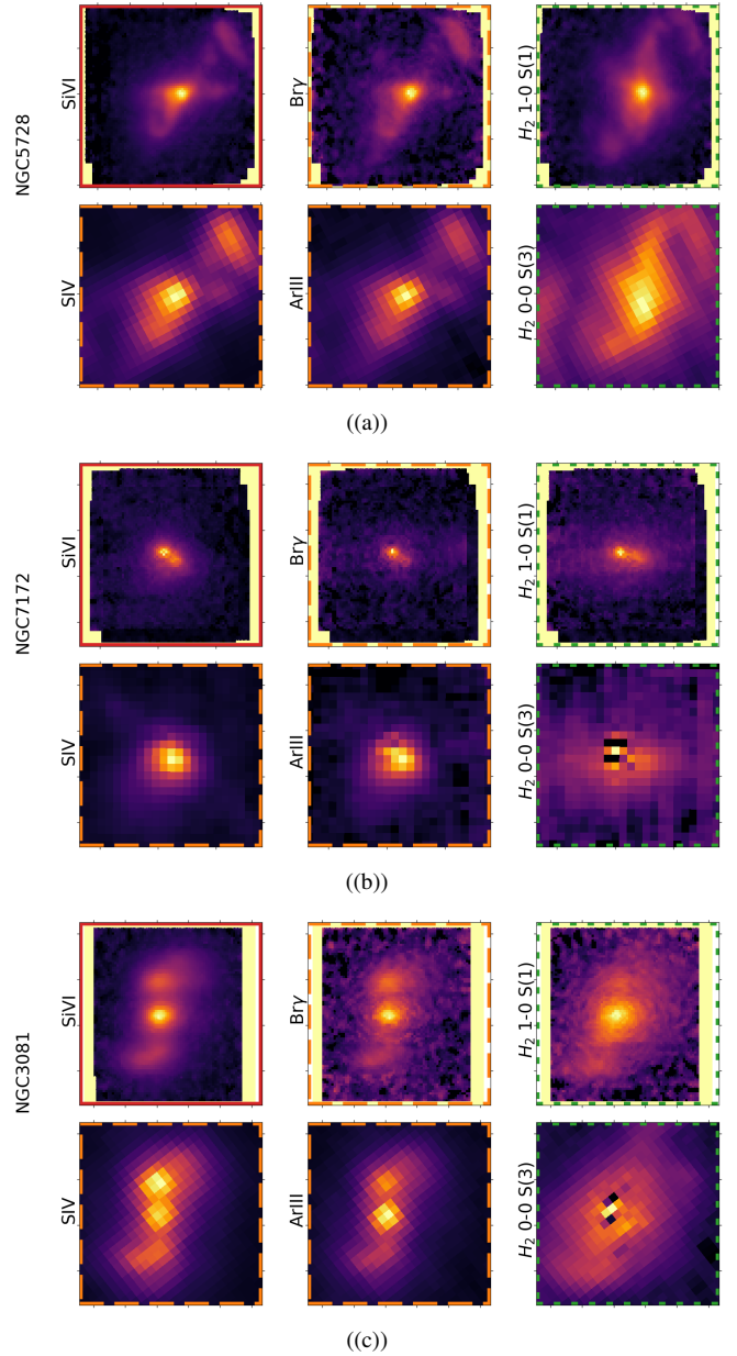
Figure A1. Linemaps for each of the shared objects, showing the lines used from SINFONI (top row) alongside the lines which are contaminating F1000W (bottom row) from MRS data. The tracer which is used for each contaminating line are shown by the colored dashed lines framing the linemaps. These maps are normalised by their total flux, and shown with a square-root stretch so as to allow visual comparison of the morphologies in order to assess the suitability of each species as a morphological tracer for the other. We note the artifacts present in the H_2 0-0 S(3) maps derived from the MRS data, which are due to the weak line being overshadowed by the "wiggles" in the continuum caused by instrument effects. These maps are not used directly at any point of this work, and are shown here for qualitative morphological comparison only.
