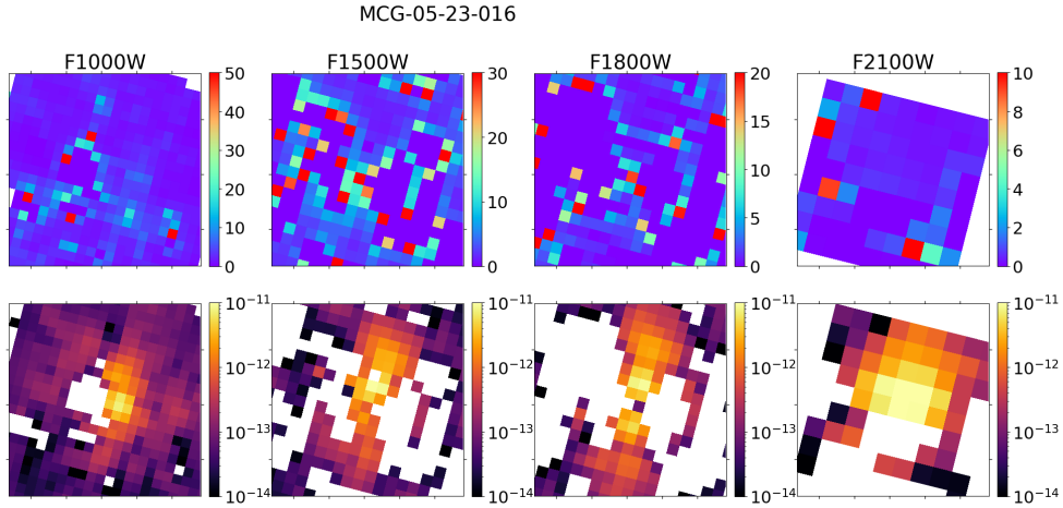
Figure C3. Contamination maps (top row) and line-free synthetic images (bottom row) shown across the 4 filters for MCG 05-23-016. These were generated using the MRS-only method described in Section 3.2.
