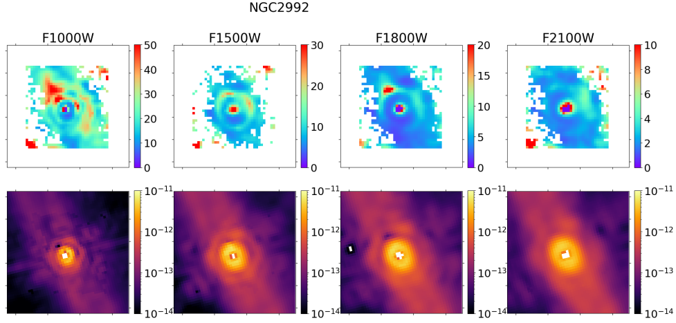
Figure C4. Contamination maps (top row) and line-free synthetic images (bottom row) shown across the 4 filters for NGC 2992. These were generated using the imaging-only estimation method described in Section 3.4, with the tracers used for the relevant lines in other bands described in Section C2.
