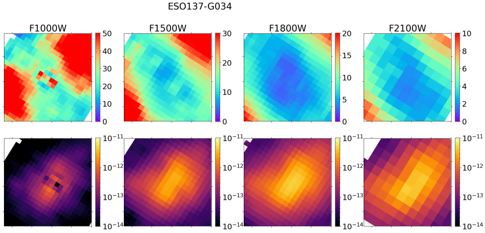
Figure C2. Contamination maps (top row) and line-free synthetic images (bottom row) shown across the 4 filters for ESO 137-G034. These were generated using the MRS-only method described in Section 3.2.
