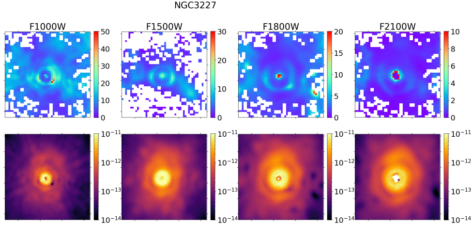
Figure C5. Contamination maps (top row) and line-free synthetic images (bottom row) shown across the 4 filters for NGC 3227. These were generated using the imaging-only estimation method described in Section 3.4, with the tracers used for the relevant lines in other bands described in Section C2.
