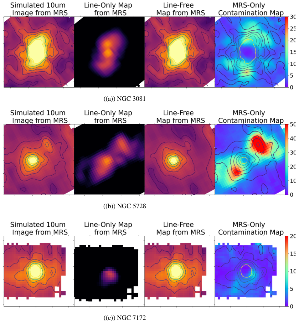
Figure B1. Results of using the MRS-only method without mitigation of the PSF on the three shared objects in F1000W – NGC 3081, NGC 5728, NGC 7172. From left to right, the full image is synthesised from the MRS data, and can be decomposed into line-only emission and line-free emission. In this case, the synthetic line-free map is effectively the decontaminated image. The contamination map is the percentage of flux in the line-free map compared with the synthetic image. The contours in these images, in all cases, represent the flux. The contours in the first column shows the flux in the image. The contours in the third column are that of the flux in the decontaminated map. The contours in the fourth column are those of the flux in the initial image.
