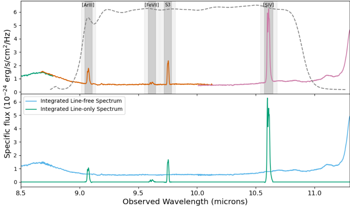
Figure 3. Top: spatially integrated spectrum from the MIRI MRS "spanned cube" for NGC 5728, showing the different gratings in green, orange and pink; overlaid in dashed grey is the MIRI F1000W broadband filter throughpass curve. Emission lines which contribute to flux within the filter range are marked and labelled. Bottom: the same spatially integrated MIRI MRS spectrum, this time decomposed into the emission line-only spectrum (green) and the line-free spectrum (blue) to illustrate the method described in Section 3.2.
