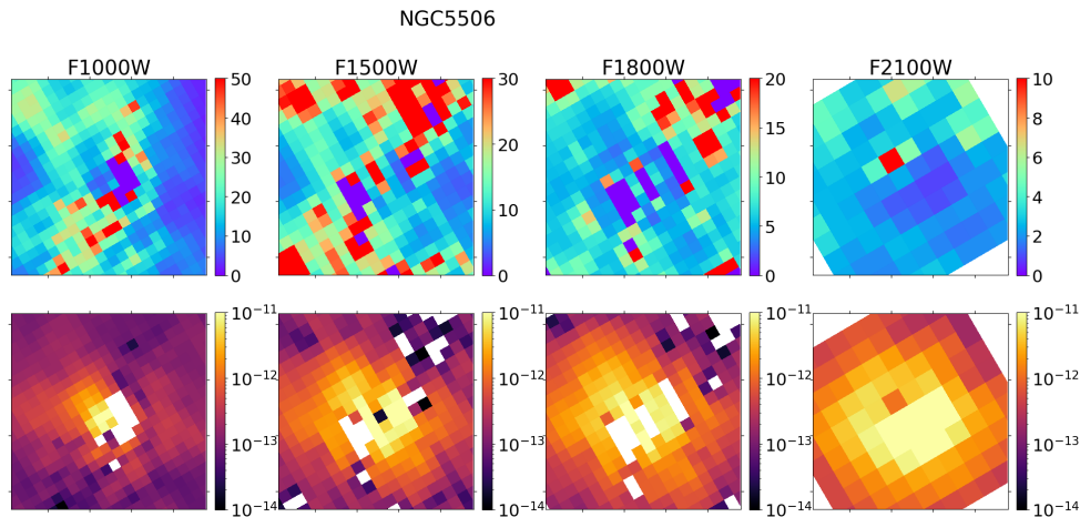
Figure C1. Contamination maps (top row) and line-free synthetic images (bottom row) shown across the 4 filters for NGC 5506. These were generated using the MRS-only method described in Section 3.2.
