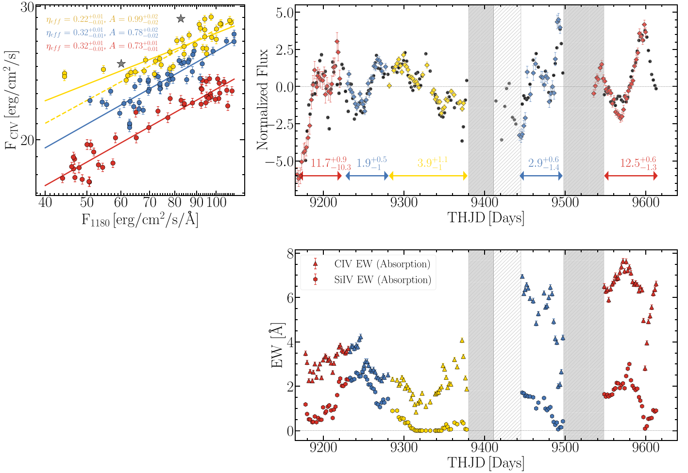
Figure 5. Upper left: Time-delay-corrected fluxes for F_{\text{CIV}} (in units of 10^{-13} \text{ erg s}^{-1} \text{ cm}^{-2} \text{ Å}^{-1} ) vs. the F_{1180} continuum (in units of 10^{-15} \text{ erg s}^{-1} \text{ cm}^{-2} \text{ Å}^{-1} ) plotted on a logarithmic scale (similar to Figure 3 but with a different color coding). The color coding represents the three main trends in the C IV emission-line response to continuum variations in Table 3. The best-fit slope to each trend is illustrated with a colored line representing the emission-line responsivity, \eta_{\text{eff}} and A is the best-fit line intercept, as given in the upper left corner (see Equation (3)). The gray stars from archival measurements (uncorrected for time delays) of Mrk 817 obtained in 2009 suggest a significantly higher response and EWs at that time. The yellow dashed line is the fit excluding the three outlier data points in the gold data points. Upper right: The continuum flux F_{1180} (black symbols) overplotted on the F_{\text{CIV}} light curve (colored symbols) where each light curve is normalized to a median of zero and an NMAD of one and also corrected for the mean time delay in each separate window. Major gaps due to HST safing events are identified by the gray shaded regions. The C IV light curve exhibits a varied behavior in response to the continuum, with the red light-curve segments showing a lag of \sim 11 –12.5 days, the blue segments a lag of \sim 2.5 days, and the gold segment a lag of \sim 4 days. Lower right: Time series of the absorption as indicated by Si IV and C IV. Each interval is color coded by the same colors as the light curve. The horizontal line shows the absorption level at zero. The gold symbols correspond to the window where the absorption is at a minimum.
