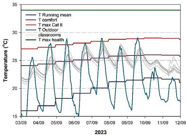
Fig. 5. Response of brick designed to Passivhaus principles, 2 storey school during September 2023 heatwave (school week: 04/09 Monday – 08/09 Friday).
