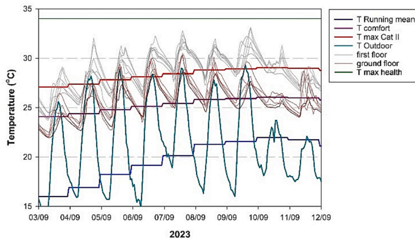
Fig. 6. Response of 2 storey SCOLA system school during September 2023 heatwave (school week: 04/09 Monday – 08/09 Friday).
