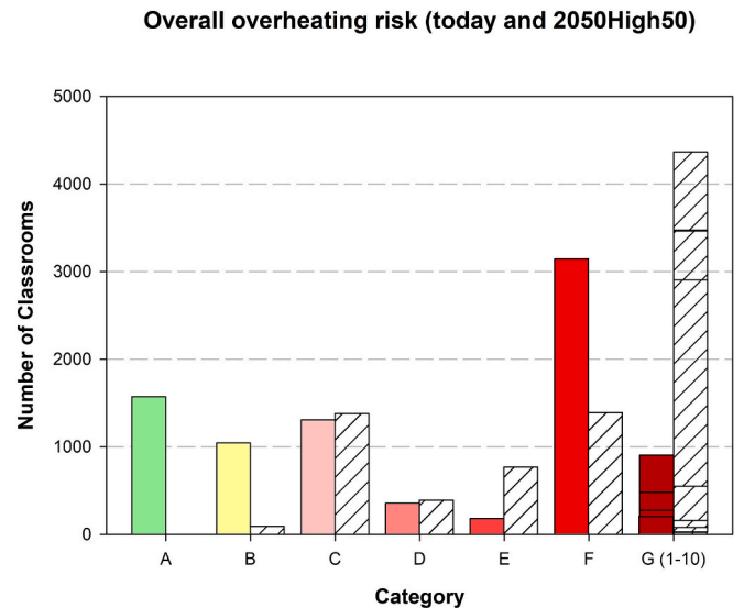
Fig. 10. Overall weighted overheating risk assessment for present state and 2050 future climate (hatched) all schools as location Swindon DSY1 50th percentile 2050. The G classification has 10 sub-bands which are stacked together (from G1 lowest to G10 most severe).
