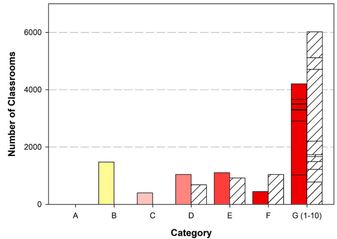
Fig. 7. Cognitive risk assessment for present state and 2050 future climate (hatched) all schools as location Swindon DSY1 50th percentile 2050. The G classification has 10 sub-bands which are stacked together (from G1 lowest to G10 most severe).
