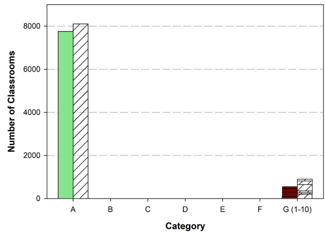
Fig. 9. Health risk assessment for present state and 2050 future climate (hatched) all schools as location Swindon DSY1 50th percentile 2050. The G classification has 10 sub-bands which are stacked together (from G1 lowest to G10 most severe).
