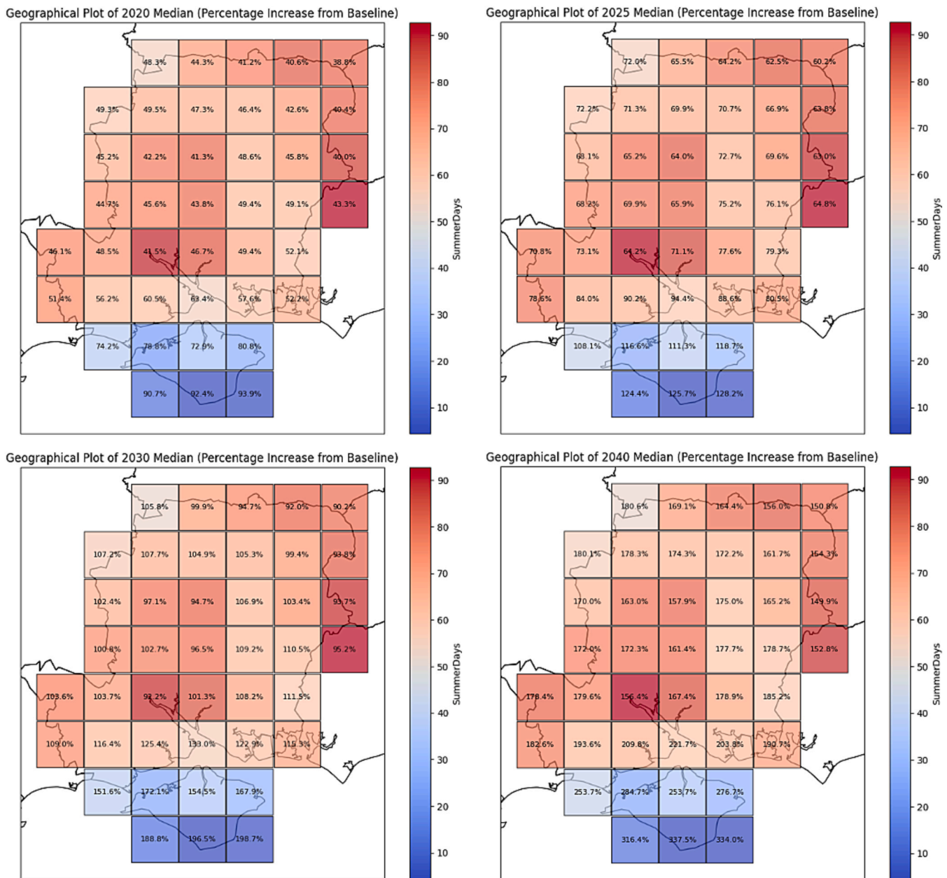
Fig. 1. Percentage increase in number of hot summer days (peak temperature > 25°C) from the baseline (2001–2020 median) in Hampshire at 12x12 km gridsquare resolution for 2020, 2025, 2030 and 2040 – Colour grid square represents the number of days above baseline.
