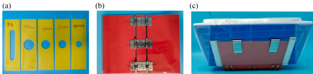
Fig. 5. Downscaled physical model with replaceable orifice plates and torsional spring fixture. (a) Orifice plates. (b) Torsional stiffness fixture. (c) Stiffness plate inserted and clipped into a frame holder on the exterior wall of the flaps.
