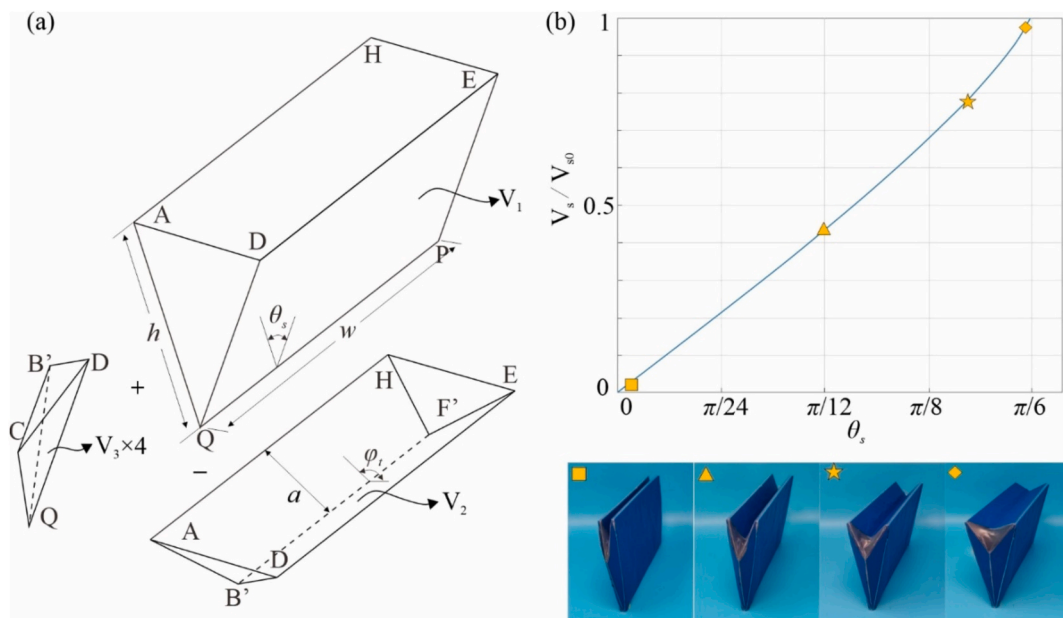
Fig. 3. (a) Single origami section decomposed into three components; the volume is calculated by subtracting V_2 from V_1 and adding 4 V_3 . (b) Normalized volume of a single origami section as a function of section angle \theta_s .
