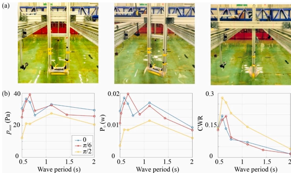
Fig. 9. (a) Physical prototype placed at different orientations relative to the incident wave direction in the coastal basin. Left to right: 0, \pi/6 and \pi/2 rad with respect to the wave front. (b) WEC performance at different orientations to the wave front.
