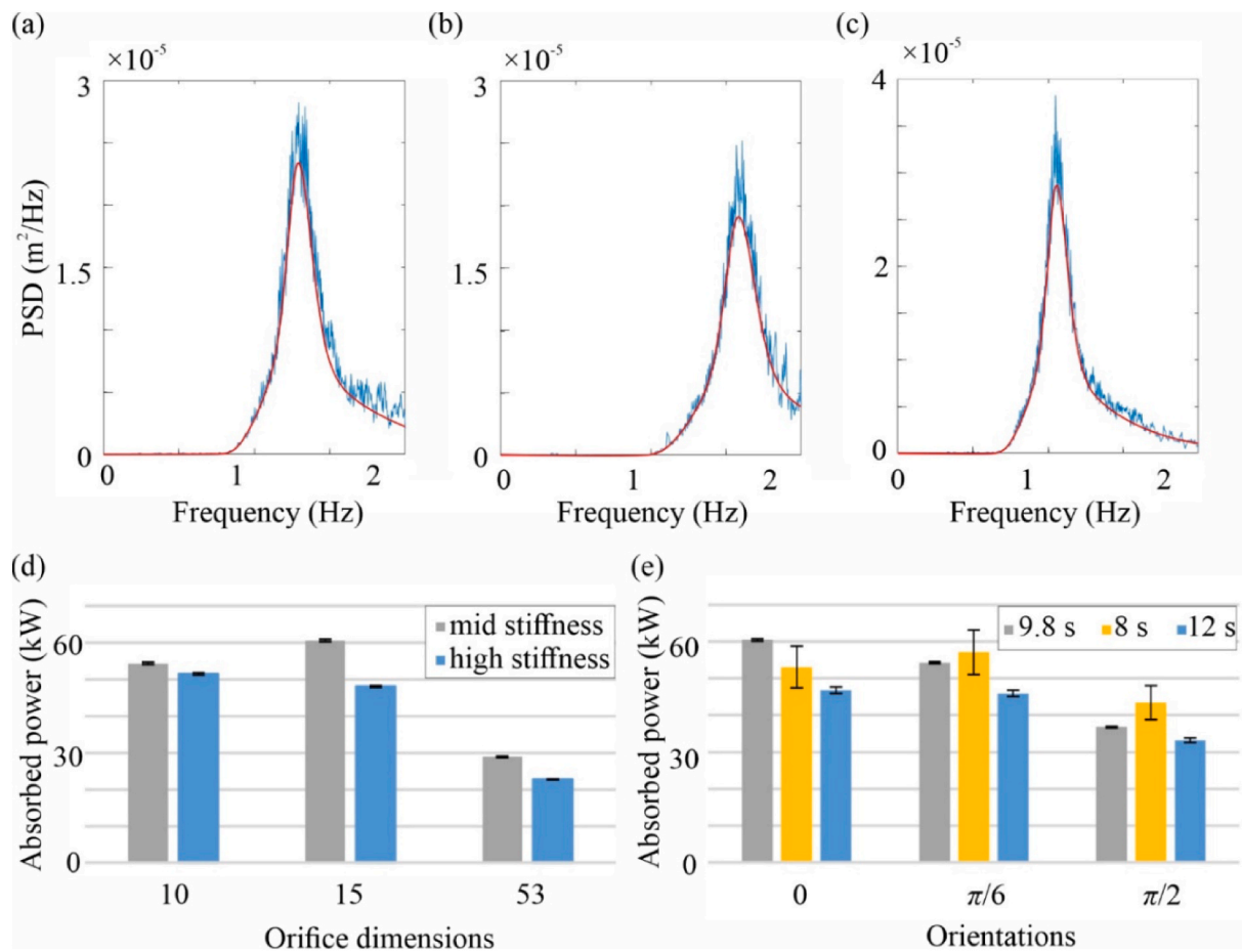
Fig. 10. Scaled irregular wave tests. Free surface elevation spectra for (a) H_s = 2 m, T_p = 9.8 s, error = 0.54 %, replicating conditions at the Wave Hub site; (b) H_s = 2 m, T_p = 8 s, error = 10.64 %; and (c) H_s = 2 m, T_p = 12 s, error = 1.87 %. Red curves correspond to expected wave profiles and blue curves to measured wave probe data from empty basin tests. (d) Histograms of absorbed power for the scaled-up model in irregular sea states replicating those at the Wave Hub site, for different values of hinge stiffness and orifice dimension, and (e) various orientations to irregular waves at different peak wave periods.
