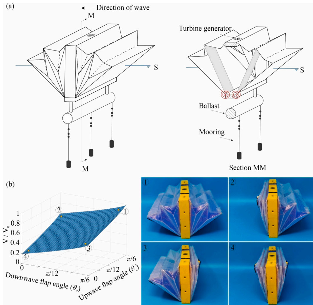
Fig. 4. WEC Design. (a) Isometric and cross-sectional views of the WEC. (b) Normalized chamber volume as a function of downwave and upwave flap angles, with photographs showing corresponding configurations of the downscaled physical prototype.
