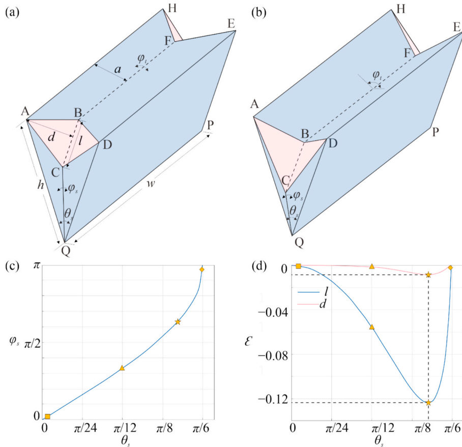
Fig. 1. Small-strain origami-inspired bellow section in (a) fully expanded state, and (b) a partially folded state. Rigid facets are in blue whereas elastic membranes are in red. The dotted lines denote valley creases, and solid lines are mountain creases. (c) Kinematic relationship of the rigid-foldable origami skeleton. (d) Membrane strain along two orthogonal directions during the folding process.
