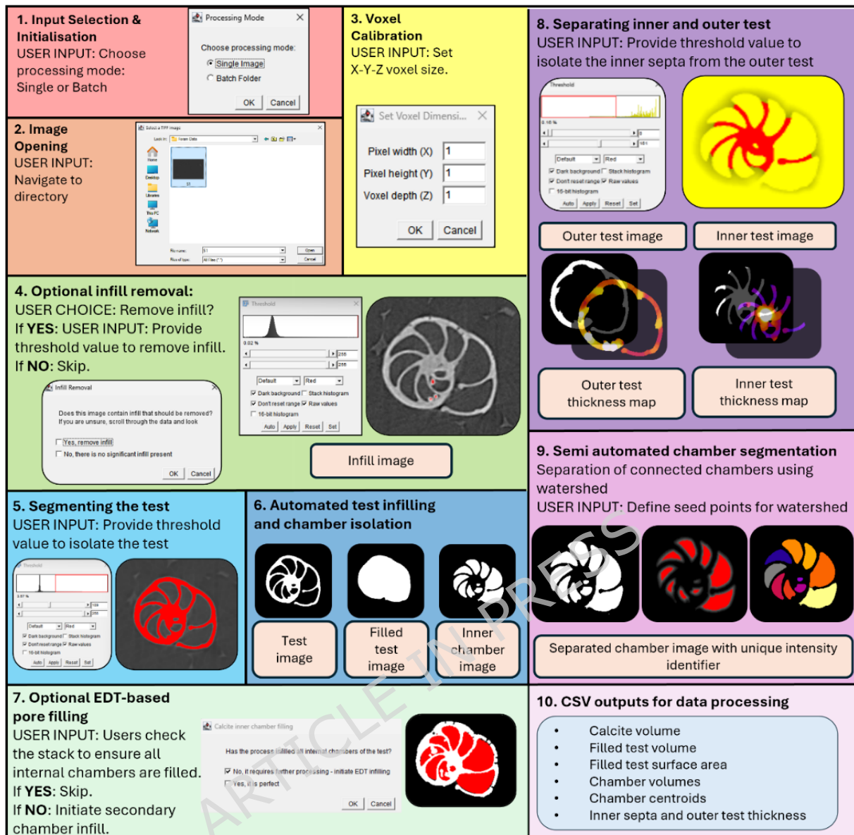
Figure 2 – Foraminiferal workflow for segmentation and morphometric analysis of foraminiferal \mu CT datasets.
