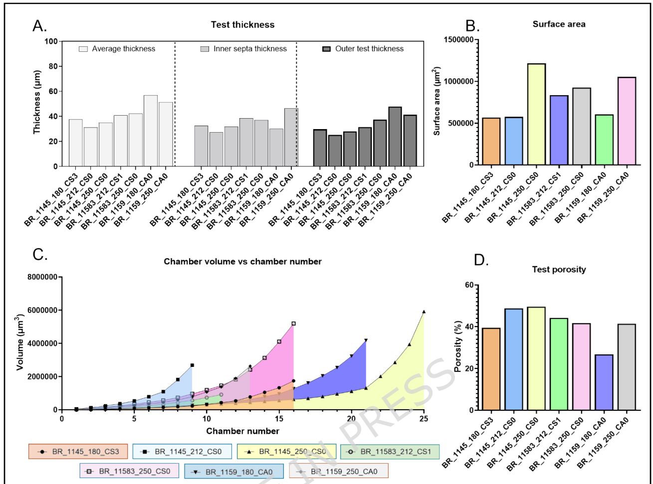
Figure 5 – Quantitative morphometric measurements derived from \mu CT-based segmentation of benthic foraminiferal tests.
