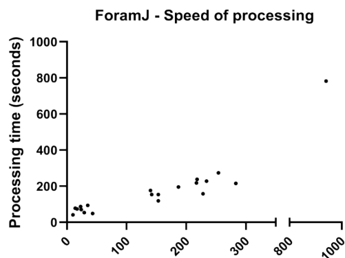
Figure 7: ForamJ processing speed. Dataset size (MB) is plotted against processing time (seconds), showcasing the scalable relationship even on low-capacity workstations.
