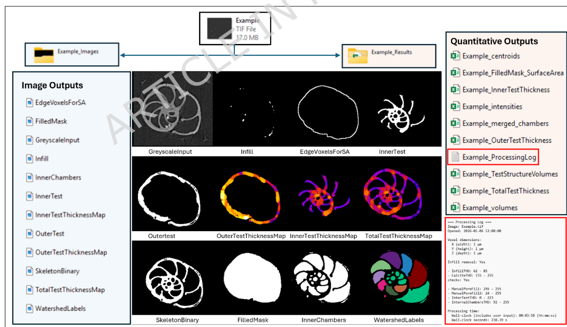
Figure 3 – ForamJ Output format
