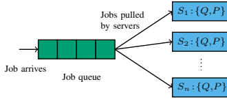
Fig. 2. Overview of JAMS.
