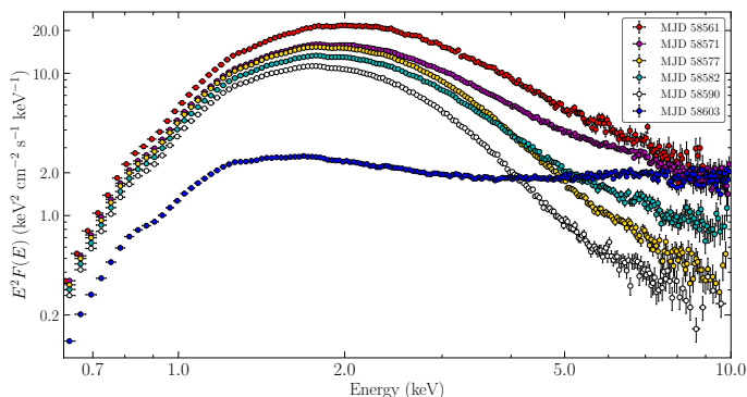
Fig. 3: NICER 0.6–10 keV unfolded energy spectra associated to the PSDs shown in Figure 2, with the same color-code. The unfolded spectra, dominated by the disk component, have been deconvolved against a power law with \Gamma = 2 , without any fitting, and are shown for illustrative purposes. We note that the spectra with broadband noise (magenta and cyan points) have slightly harder tails at high energies than spectra without variability (e.g. yellow and white points), supporting the scenario in which the variability is connected to the hot corona, which may disappear in the aftermath of a discrete ejection.
