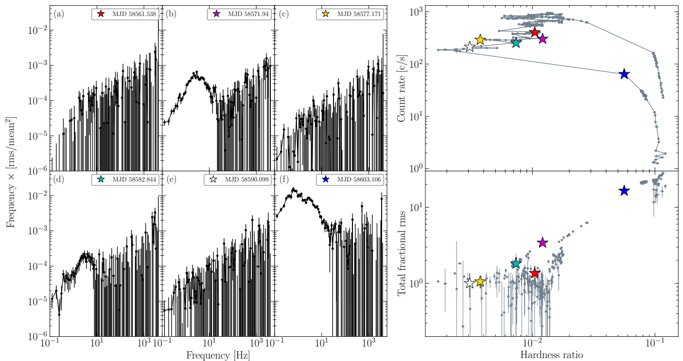
Fig. 2: Left panels : Representative NICER power spectra at different phases of the outburst, calculated in the 0.5–12 keV band and labeled from a to f . Right panels : NICER hardness-intensity diagram (HID, top) and hardness-rms diagram (HRD, bottom) of the outburst. The hardness ratio is calculated as (6 - 12)/(2 - 3.5) keV, while the total fractional rms is calculated in the 0.5–64 Hz frequency range (and 0.5–12 keV energy range). In both rows, the colored stars mark the position in the diagrams at which the power spectra were obtained. The presence of strong band-limited noise typical of the hard state supports the reactivation of compact jets during the short HIMS phase around MJD 58570. The two drops in X-ray rms variability happening after 58576 and after MJD 58582 could be consistent with the launch of the RK2 and RK3 discrete ejecta, respectively.
