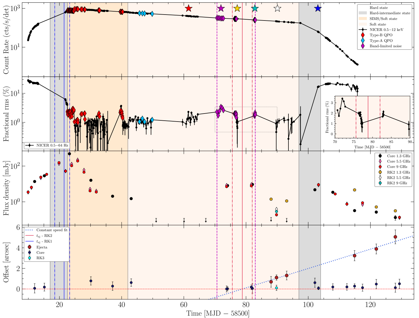
Fig. 1: Top panel : NICER 0.5–12 keV X-ray light curve (count rate) of MAXI J1348–630 during its 2019/2020 outburst. The white, light-gray, light-orange and light-pink regions denote, respectively the hard, HIMS, SIMS and soft state, from Zhang et al. (2020). The purple vertical dashed lines region marks the presence of intermittent strong band-limited noise during the soft state. Type-B and A QPOs are marked with red and light-blue points, respectively. The colored stars mark the times in the light curve at which the power spectra shown in Figure 2 were obtained. Second panel : X-ray fractional rms variability, calculated in the 0.5–64 Hz frequency range. The inset on the right shows in detail the evolution of the variability between MJD 58570 and 58590. Third panel : MeerKAT (1.3 GHz) and ATCA (5.5 and 9 GHz) core and RK2 radio light curves, from Carotenuto et al. (2021). Bottom panel : Angular separation in arcsec between RK2 and MAXI J1348–630 from the same radio observations. Detections of the core are shown as dark blue points. The single detection of RK3 is also marked with a cyan point. A linear motion was used to fit the RK2 data. The red vertical line marks the RK2 inferred ejection date: t_{ej} = \text{MJD } 58578.8 \pm 3.2 , where the two red dashed lines represent the upper and lower bounds of the t_{ej} confidence interval. The same is shown in blue for RK1, with t_{ej} = \text{MJD } 58521.5^{+1.8}_{-3.0} from Carotenuto et al. (2022).
