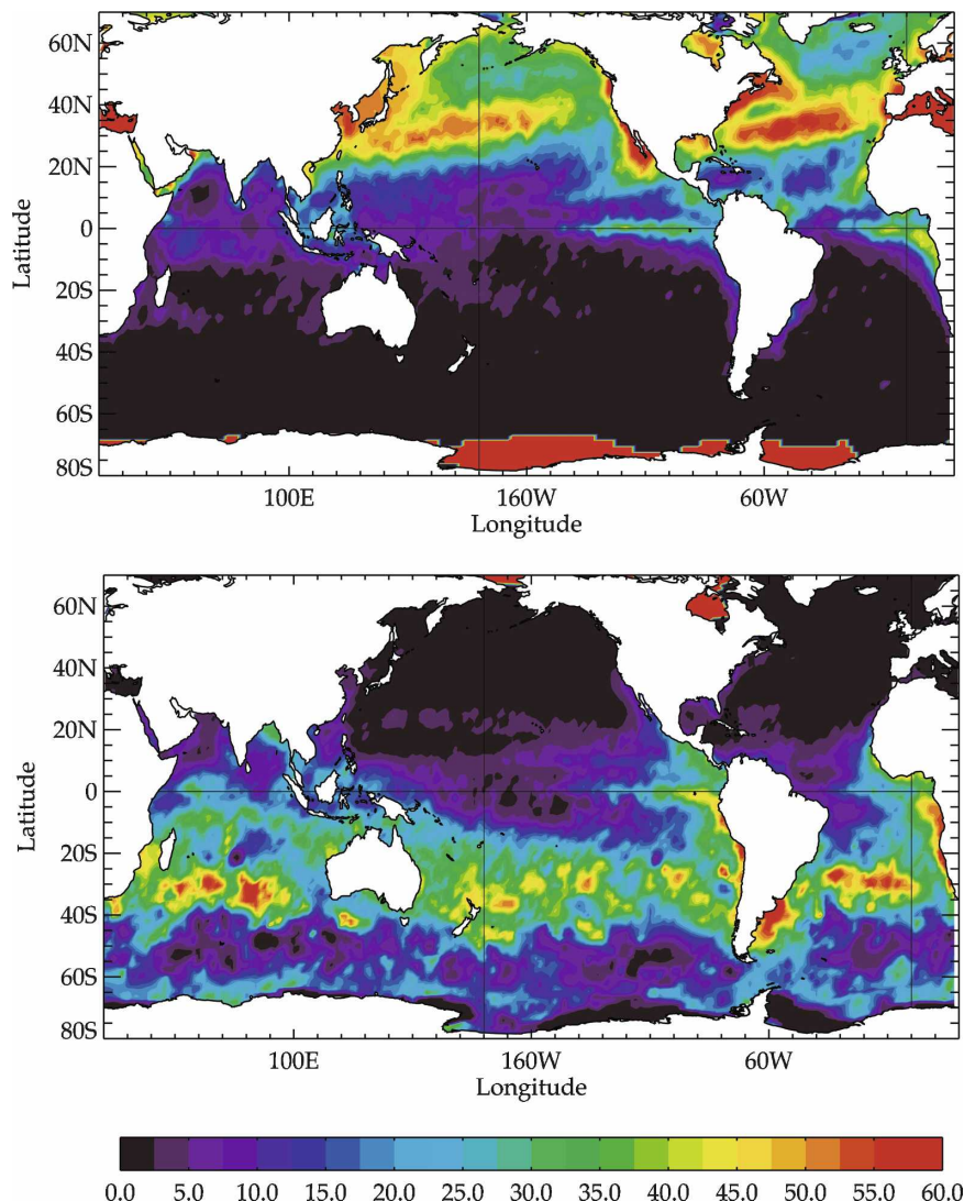
FIG. 2. Mean shortwave radiation ( W m^{-2} ) at the base of the mixed layer in (top) July and (bottom) January. Solar irradiance at the surface is derived from the standard bulk formulas and climatological cloud cover used to force the model (see Iudicone et al. 2008). Solar irradiance is assumed to be attenuated as in the standard clear-water double-exponential formulation, with e -foldings of 0.35 and 23 m for the near-IR and visible wavelengths, respectively [the same formulation is used in the ice-ocean model; e.g., Manizza et al. (2005)]. A recent climatology is used for the estimate of the mixed layer depth (de Boyer Montegut et al. 2004). A significant warming of the base of the mixed layer is observed in the tropics in both seasons (see also Siegel et al. 1995), while extratropical regions are warmed only during summer (see also Ohlmann et al. 1996).
