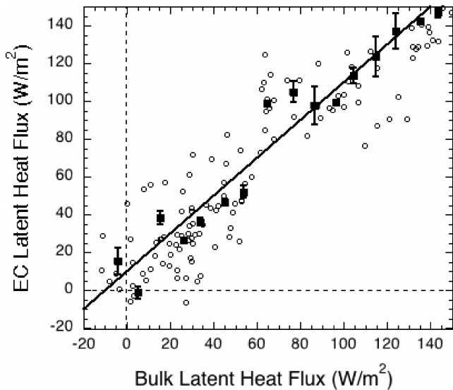
Fig 7: EC latent heat fluxes against bulk formula 23 estimates. Individual 1h samples (o) and average (■) results per 10 W/m 2 bin (error bars are ± 1 sd) are shown. The solid line shows the linear regression of the averaged results
