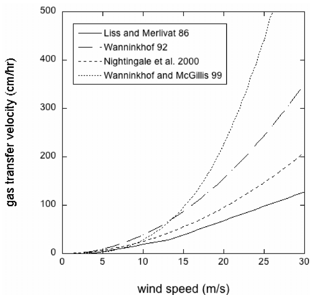
Fig 1: Parameterisations 7,8,9,10 of the gas transfer velocity, k , in terms of the mean wind speed from various studies as given in the key. Note that no direct measurements of k have been made for winds over 15m/s
