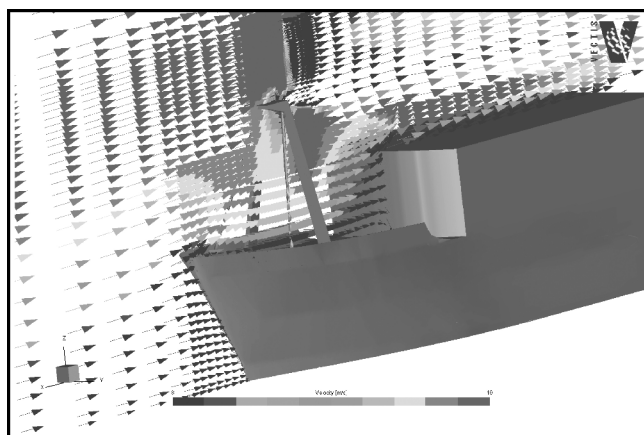
Fig 3: A slice of data from a 3-D computational fluid dynamics simulation of the air flow over a very simplified representation of the Polarfront
