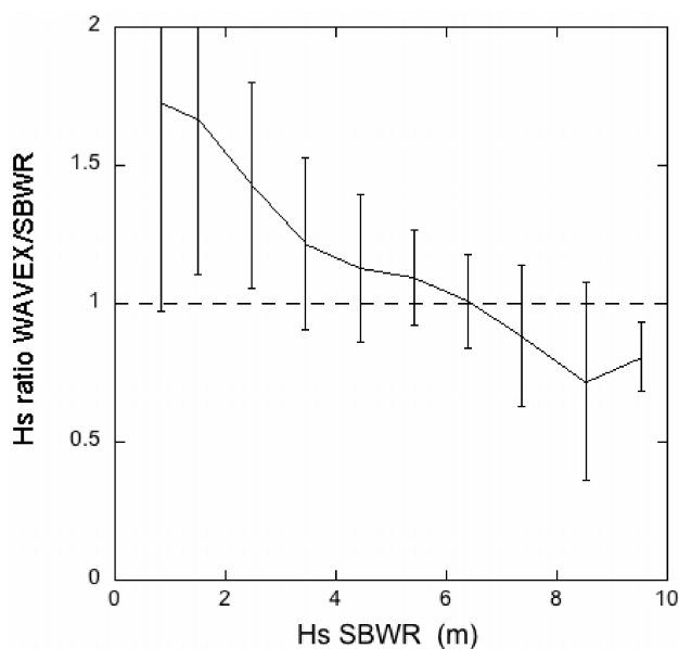
Fig 9: Averaged WAVEX:SBWR ratio for significant wave height (Hs). The dashed line indicates 1:1 agreement
