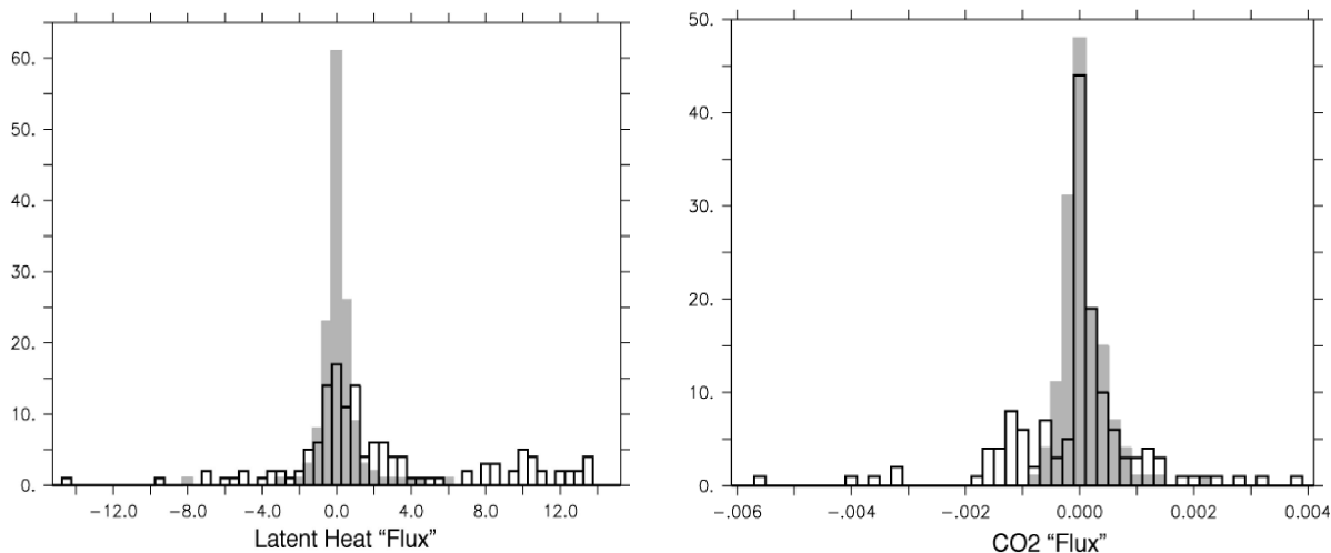
Fig 6: Latent heat (left, W/m^2 ) and CO_2 (right, mmol/m^2.s ) ‘fluxes’ from the shrouded Licor before (white) and after (grey) correcting for the deformation of the sensing head
