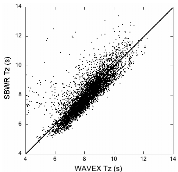
Fig 8: Hs (left) and Tz (right) from the two wave systems. The solid line indicates a 1:1 relationship
