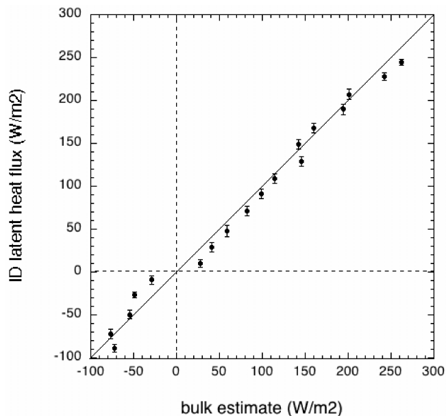
Fig 5: Latent heat fluxes ( W/m^2 ) calculated from the ID method against those estimated from a bulk formula. 23 A 1:1 line is shown
