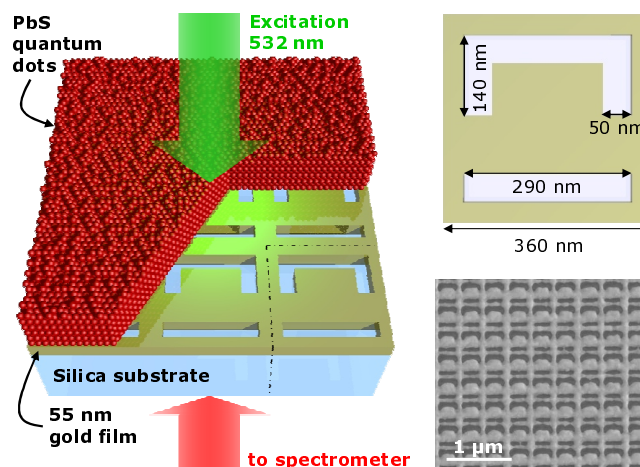
Figure 1: Photonic metamaterial hybridized with semiconductor quantum dots. The insets show the metamaterial unit cell and an SEM image of the actual metamaterial structure.
