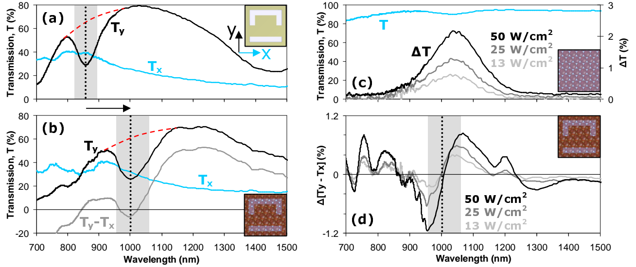
Figure 2: Transmission spectra of (a) the metamaterial before deposition of quantum dots and (b) the metamaterial after deposition of PbS quantum dots. Blue lines correspond to x -polarization, black lines correspond to y -polarization and a differential spectrum T_y - T_x is shown in gray. The trapped-mode resonance for y -polarization is marked by a gray shaded region. (c) Transmission spectrum of PbS quantum dots on a glass substrate (blue line). The resonant curves show the change \Delta T of the transmission signal due to optically pumping the quantum dot layer on the glass substrate. (d) Difference between pump-induced changes of the transmission signal for x and y -polarizations for different levels of pumping.
