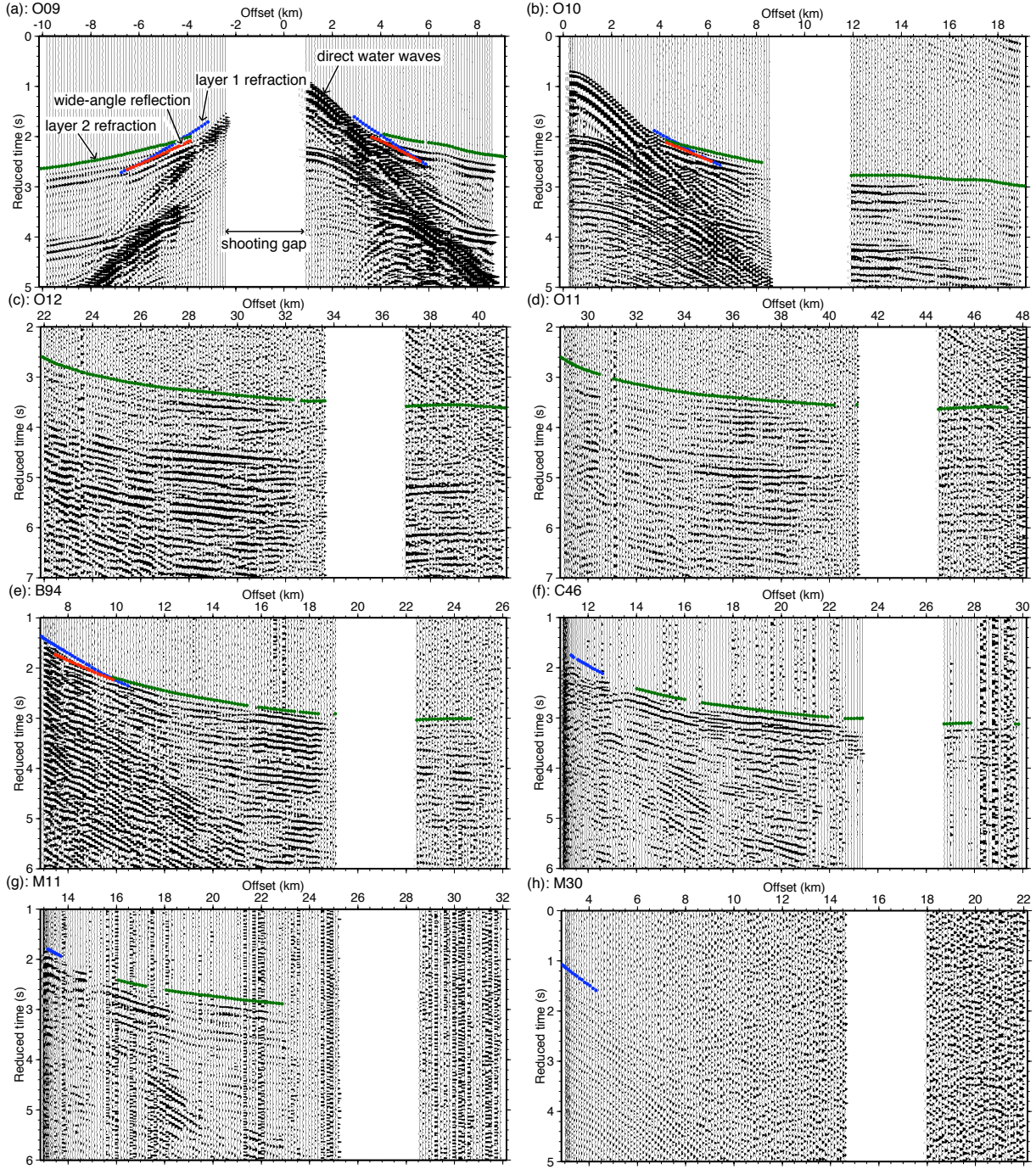
Figure 3. Examples of seismic data plotted as common receiver gathers. Panels correspond to the radial shooting line from point A (right end of the panels) to site O10 (left end) in Fig. 2 recorded on the eight instruments used in the 2D inversion. (a)-(d) Hydrophone channel recordings of OBS stations O09, O10, O12 and O11. (e)-(f) Vertical geophone recordings of Texan stations B94 and C46. (g)-(h) Vertical component recording of Reftek 130 stations M11 and M30. Synthetic traveltimes calculated through the final velocity model are superimposed on the data (blue: layer 1 refractions; green: layer 2 refractions; red: wide-angle reflections). The white gap present in all panels corresponds to an interruption in shooting due to marine mammals in the vicinity of the guns. A minimum-phase filter with corner frequencies 3-5-20-25 Hz was applied to the data. Amplitudes are normalized with a factor inversely proportional to offset.
