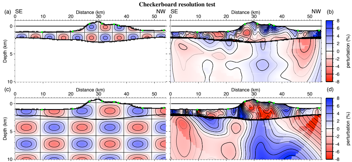
Figure 5. Results from the checkerboard resolution test. Left panels show perturbation added to the final model, right panels show recovered perturbation. (a),(b): 6.0 \times 2.0 km anomaly. (c),(d): 10.0 \times 3.0 km anomaly. Paler areas are not sampled by rays in the final inversion step. Station positions are marked by green dots. Vertical exaggeration is 2:1.
