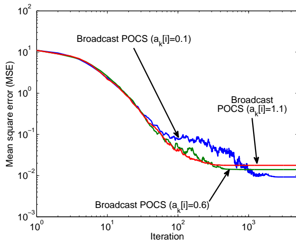
Figure 2: Transient performance of the broadcast POCS algorithm as a function of a_k[i] . Except for a_k[i] , the parameters of the algorithms are identical to those of the Broadcast POCS-d algorithm in Table 1.
