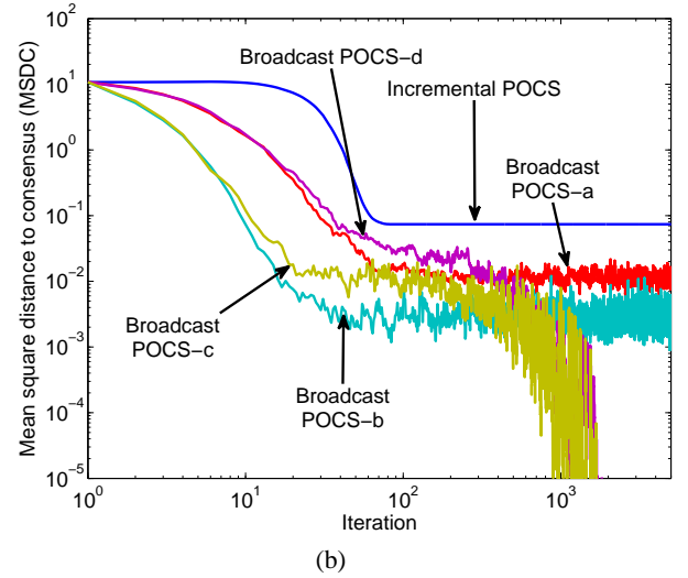
Figure 1: Transient performance of the algorithms. (a) Mean square error. (b) Mean square distance to consensus.
