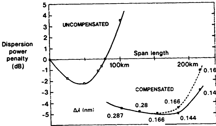
Figure 4: Receiver penalty compared to the back-to-back sensitivity of -27dBm at a 10^{-11} BER for varying span lengths.
