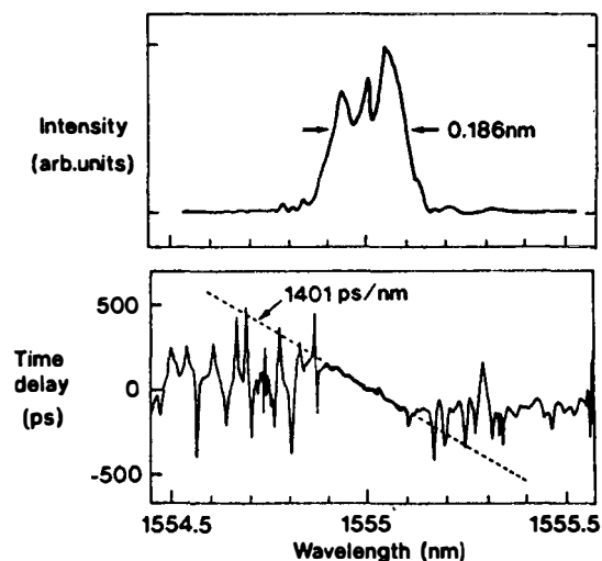
Figure 2(a,b): Typical reflection spectra and time delay characteristics measured using an interferometric test rig 6 , in this case for a temperature differential of 15^\circ\text{C}/45\text{mm} .
