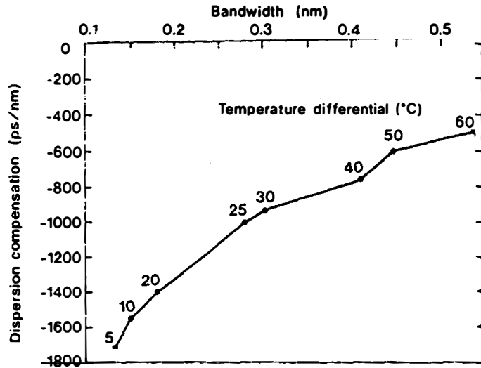
Figure 3: Measured bandwidth-dispersion characteristic for the tunable grating.
