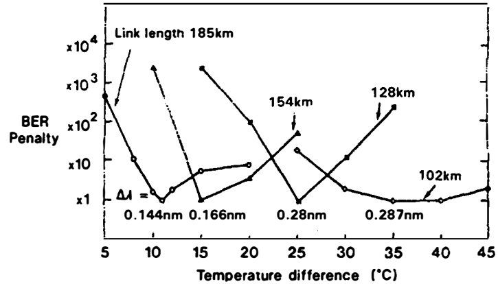
Figure 5: BER penalty as a function of temperature differential for span lengths in the range 102.6-185.3km. Results indicate the degree of dispersion tuning.
