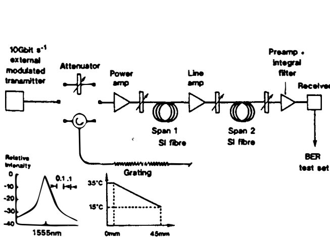
Figure 1: Experimental setup.
