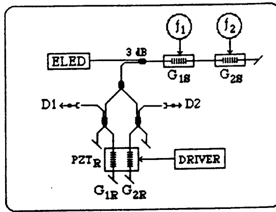
Figure 3. Experimental system with two sensor-receiving grating pairs.
