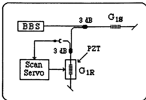
Figure 1. Basic concept of sensor receiving grating pair.
