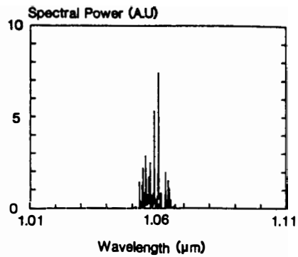
CWE6 Fig. 3. Time-averaged spectrum from the cladding-pumped fiber laser.
