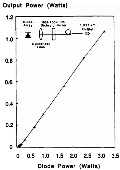
CWE6 Fig. 2. Output characteristics of the fiber laser when pumped at 808 nm with an SDL 3-W diode array.
