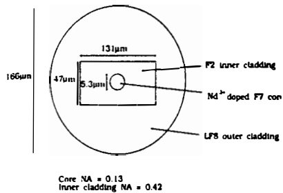
CWE6 Fig. 1. Structure of the doubly clad neodymium-doped fiber for cladding pumping.
