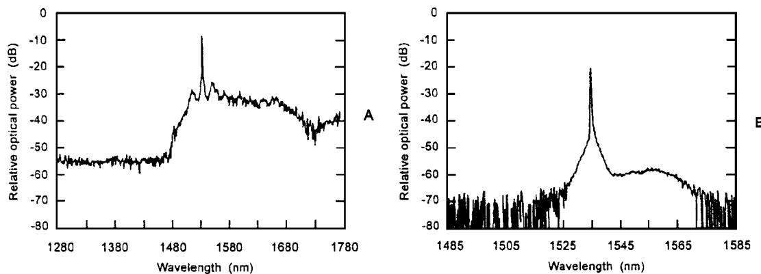
Figure 2: 100ns pulse output spectra from fibres A and B at a repetition rate of 1kHz, corresponding to pulse energies of 158 \mu J and 123 \mu J respectively.
