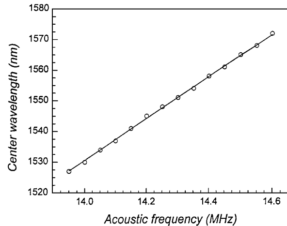
Fig.3 Filter tuning curve.
