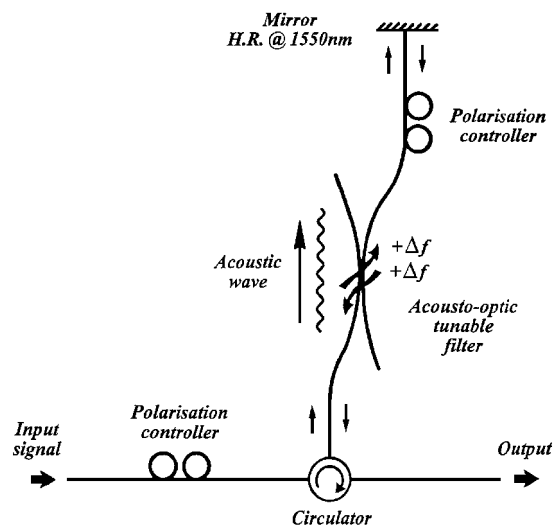
Fig. 4 Double pass filter configuration.
