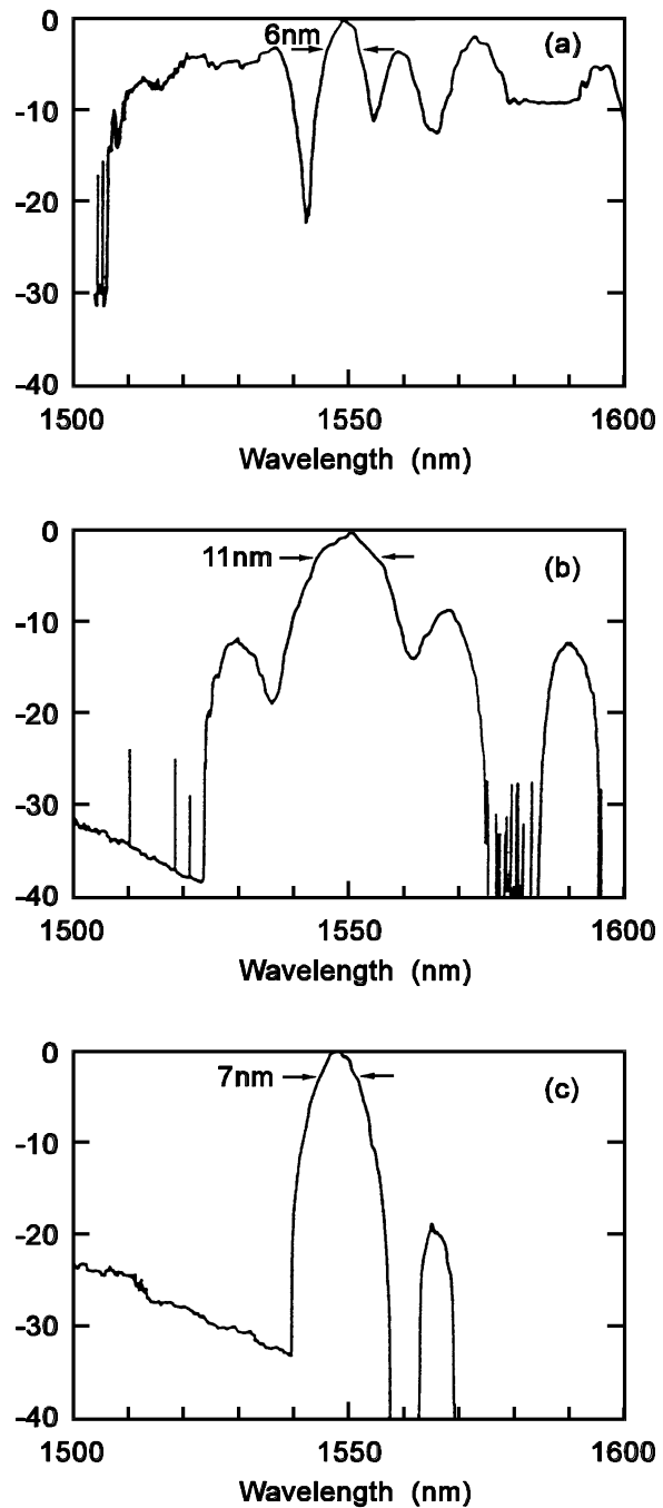
Fig.1 Coupled spectra of AO filters based on a null coupler with an interaction length of (a) 25mm, (b) 8mm and (c) 8mm with a double pass.
