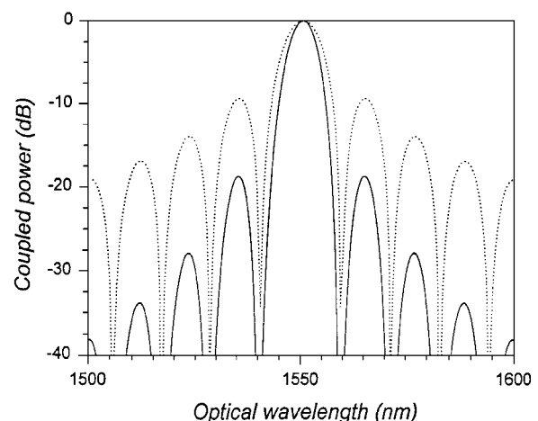
Fig. 2 Theoretical filter response of the 8mm device for (a) single (dotted line) and (b) double (solid line) pass configurations.
