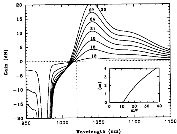
Fig. 7. Results of computer modeling, showing gain spectra for various values of launched pump powers, with the fiber length chosen to maximize available gain at 1020 nm. Optimum fiber length as a function of pump power is shown in the inset (fiber diameter 3.0 \mu\text{m} , \text{NA} \sim 0.17 , [\text{Yb}^{3+}] \sim 550 \text{ ppm} , pump wavelength 840 nm).
