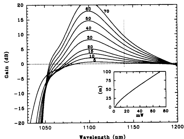
Fig. 9. Gain spectra calculated for various launched pump powers, with the fiber length chosen to maximize gain at 1140 nm as shown in the inset (fiber diameter 3.75\ \mu\text{m} , \text{NA}\sim 0.17 , [\text{Yb}^{3+}]\sim 550\ \text{ppm} , pump wavelength 1047 nm).
