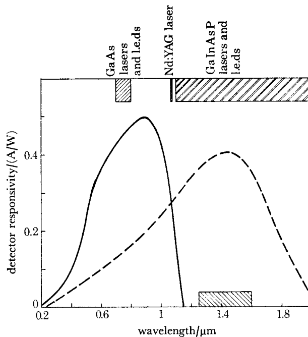
FIGURE 5. Spectral response of silicon (solid line) and germanium (broken line) photodiodes. The emission regions for various optical sources (shaded areas, top) and the region of minimum fibre attenuation (shaded area, bottom) are also shown.
