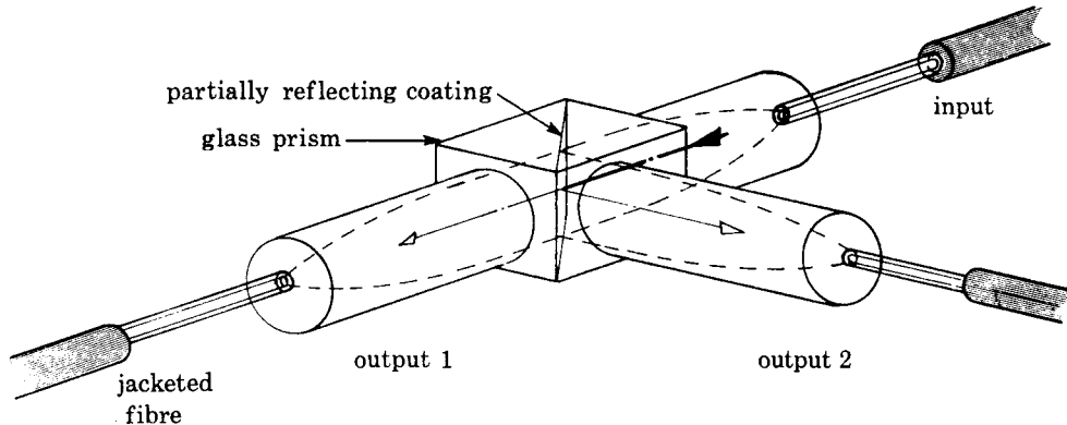
FIGURE 9. T-coupler based on Selfoc rods. The focusing rods are cut to a length which converts the divergent fibre emission to an approximately parallel beam within the central prism. Here power splitting is accomplished by a partially reflecting mirror placed at 45^\circ , after which refocusing of the beam components into the two output fibres occurs.
