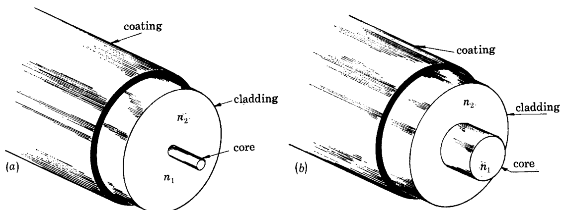
FIGURE 1. Schematic diagram of a single-mode (a) and a multimode (b) fibre showing, in each case, the core, cladding and surface-protective coating. The core diameter of the single-mode fibre is normally a few micrometres while that of the multimode fibre can be up to 100 \mu\text{m} or more.
