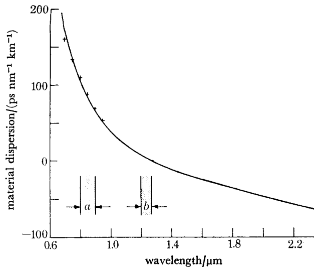
FIGURE 3. Material dispersion factor (\lambda/c)(d^2n/d\lambda^2) calculated for pure silica (solid line) and measured in a fibre having a phosphosilicate glass core (experimental points) as a function of wavelength (after Payne & Gambling 1975): a , GaAs device region; b , region of negligible material dispersion.
