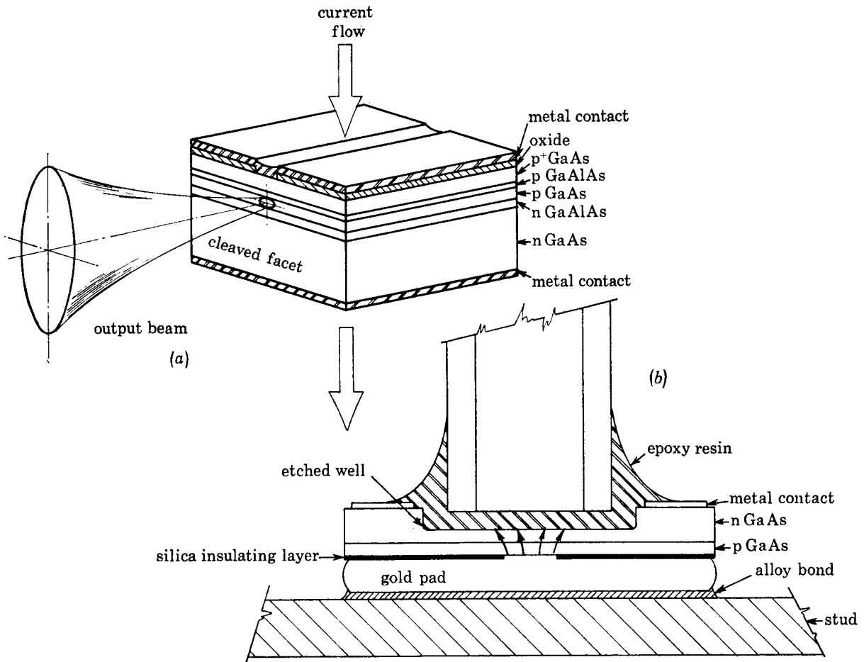
FIGURE 4. Semiconductor electroluminescent devices based on GaAs. (a) Stripe-geometry, double-heterojunction laser structure with output beam shown schematically. (b) High-brightness Burrus l.e.d. showing how the incoherent emission is coupled into a fibre.
