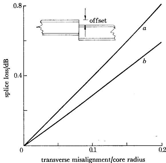
FIGURE 7. Splicing losses produced by transverse offset between fully excited multimode fibres. For a given displacement the loss is 35% larger in parabolic-index fibres ( a ) than in step-index fibres ( b ).
